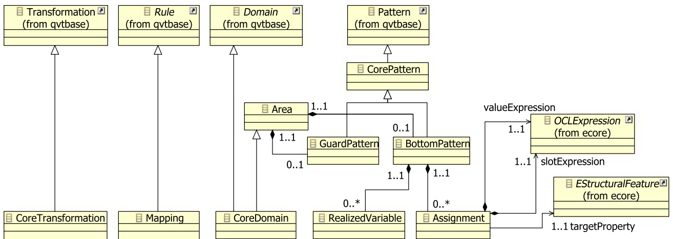
Fig. 14 The QVT-Core meta-model
