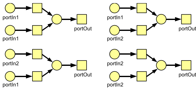
Fig. 29 The result of a MediniQVT transformation of a join component
