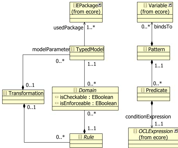
Fig. 13 The QVT-Base package
