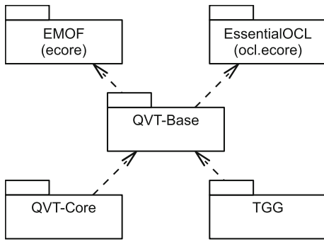
Fig. 12 The QVT-Core and TGG package dependencies
