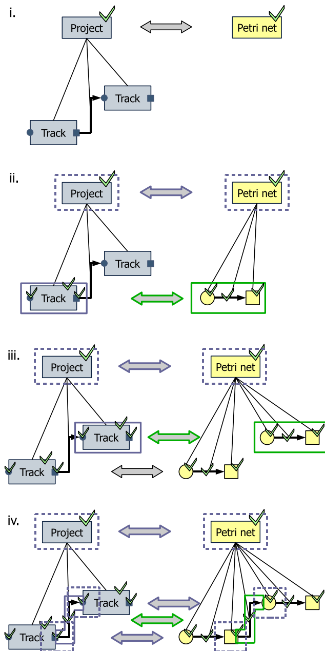
Fig. 4 Example rules: a forward transformation
