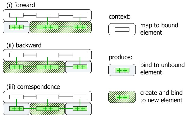
Fig. 9 The different application modes of a TGG rule and the interpretation of context/produced nodes
