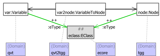
Fig. 22 Rule: VariableTypeClassToNodeTypeClass
