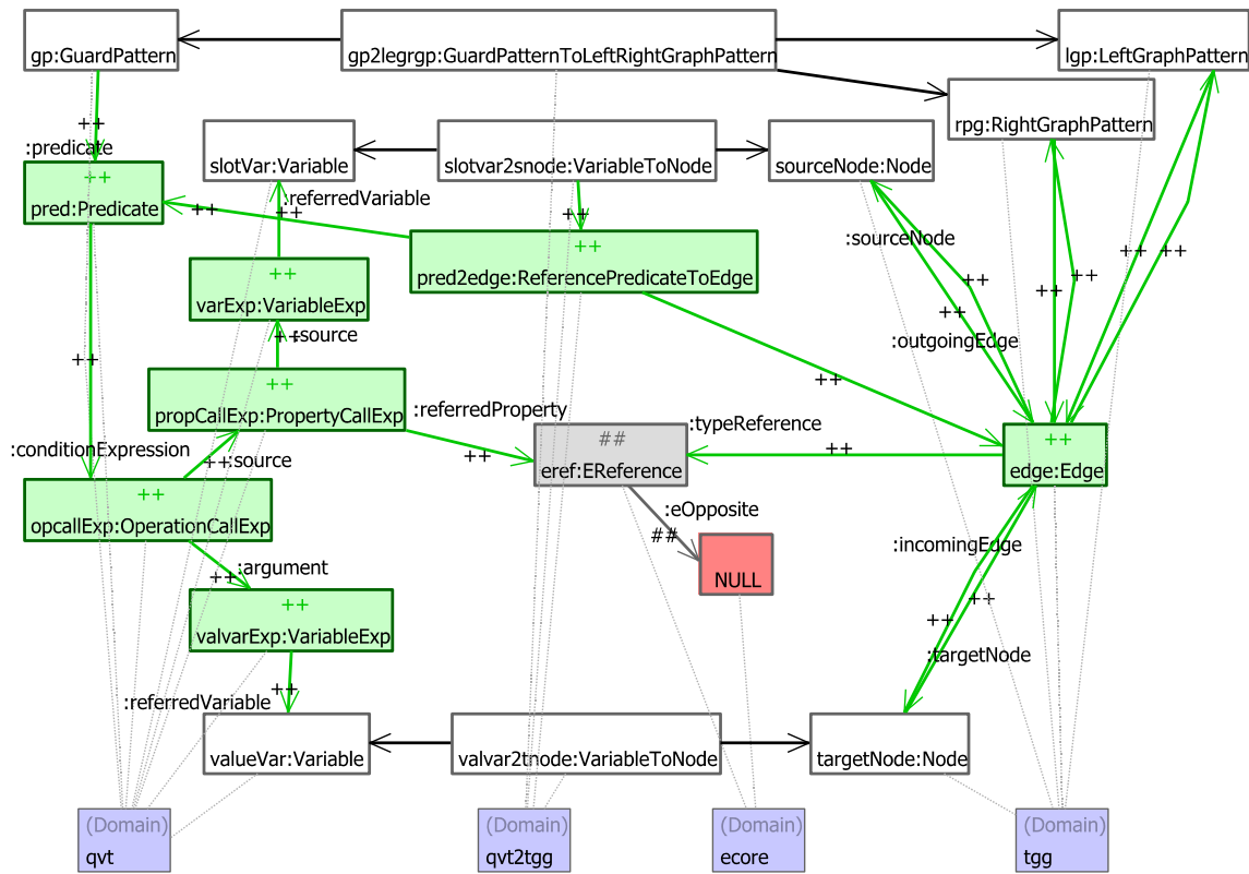
Fig. 23 Rule: ReferencePredicateToEdge
