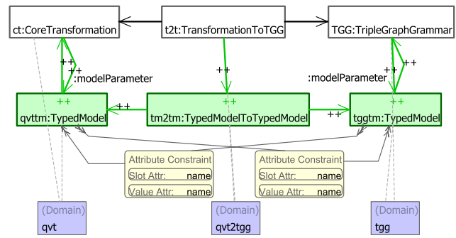
Fig. 18 Rule: TypedModelToTypedModel
