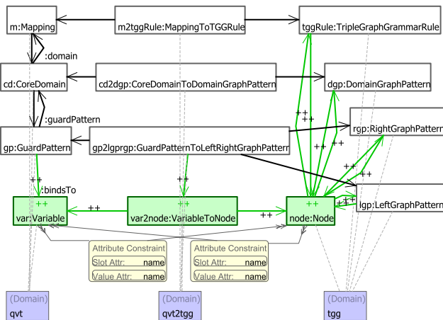
Fig. 21 Rule: GuardPatternVariableToNode
