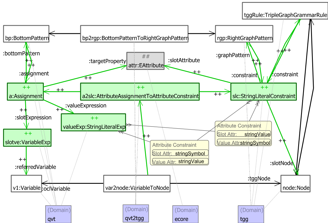
Fig. 24 Rule: StringLiteralAssignmentToStringLiteralConstraint
