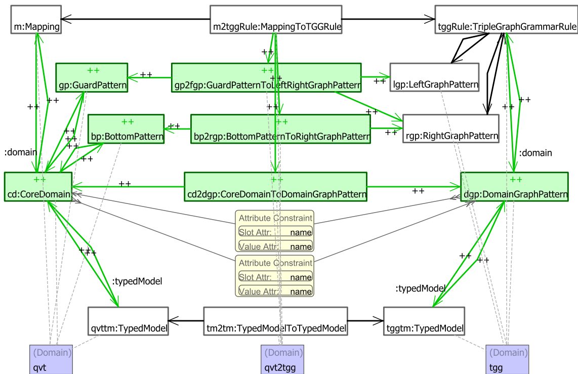
Fig. 20 Rule: CoreDomainToDomainGraphPattern
