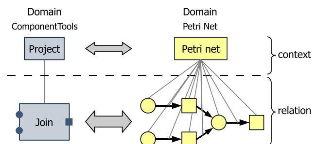
Fig. 28 Relation of a join component and its Petri net structure
