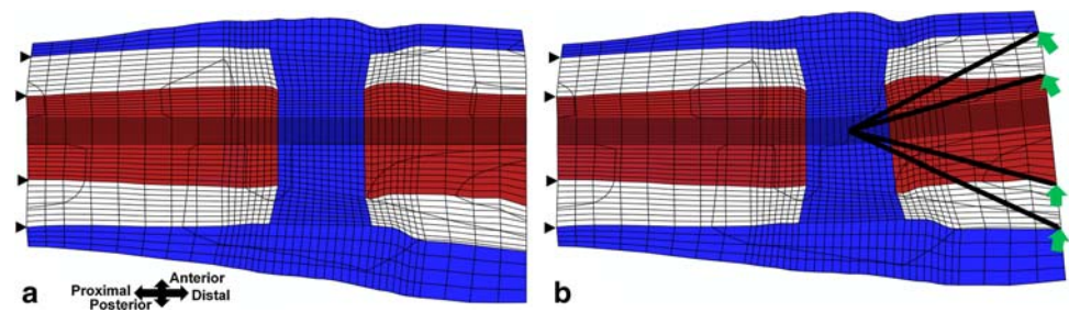
Fig. 2 Finite element mesh bent a 0^\circ and b +6^\circ about the center of the osteotomy gap in the sagittal plane. The (displacement) boundary conditions are shown
