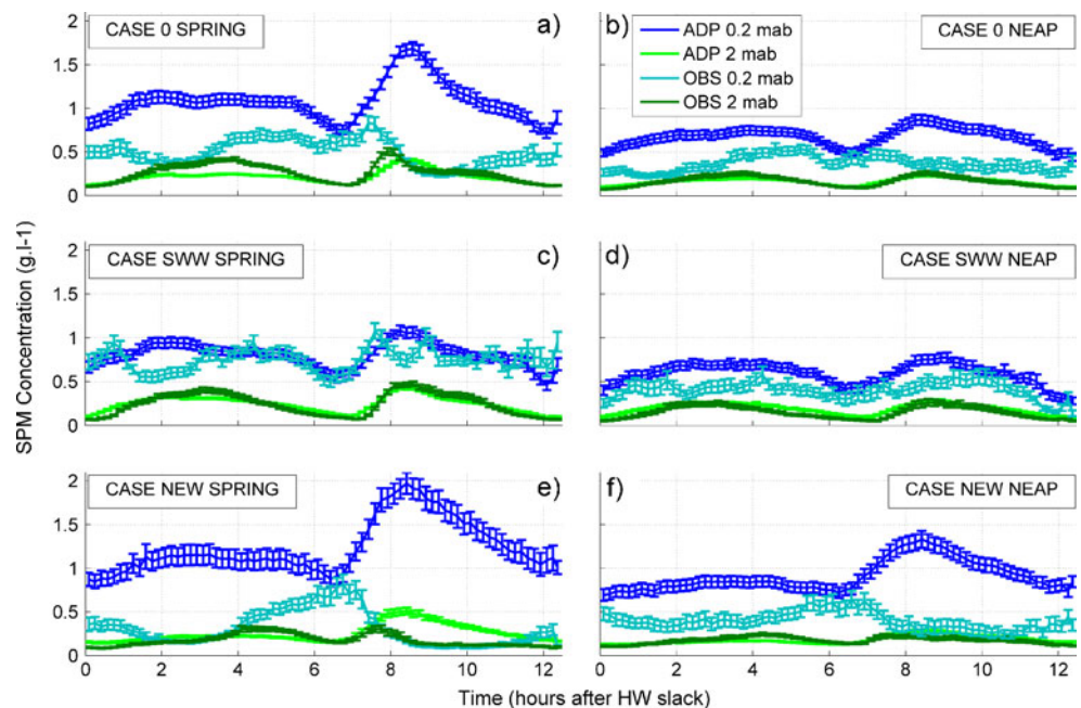
Fig. 7 Ensemble-averages of tidally varying SPM estimates from OBS and ADP at 0.2 (blue) and 2 mab (green). The error bars indicate standard error
