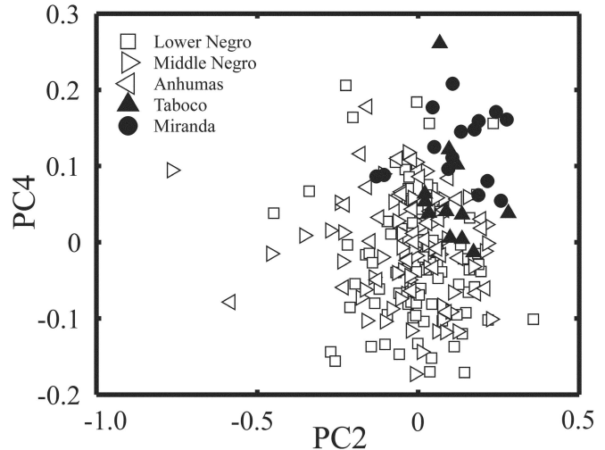
Fig. 3. Scatterplot of PC2 against PC4, categorized by region. Specimens from highland localities (Miranda, Taboco) appear as filled symbols ; those from lowland localities (Anhumas, lower Negro, middle Negro) appear as open symbols
