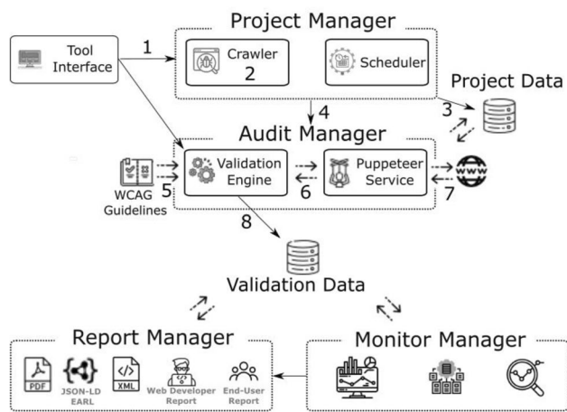
Fig. 8 The Tool Architecture
