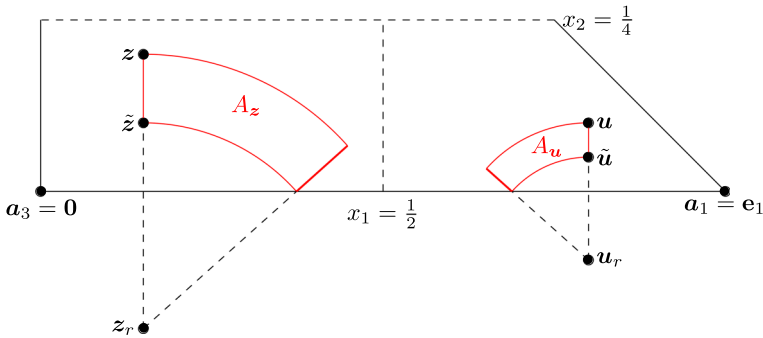
Fig. 2 Annular regions of integration (red) in the proof of (B.2), where \tilde{z} := (z_1, z_2/2) and \tilde{u} := (u_1, u_2/2) (Color figure online)
