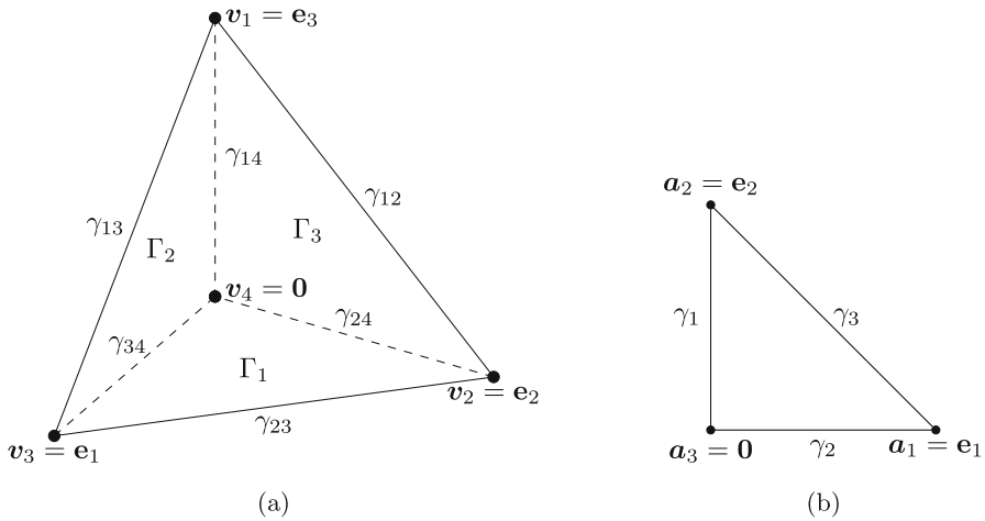
Fig. 1 Reference a tetrahedron and b triangle, where e_i are the standard unit vectors. Note that the label for \Gamma_4 = \{(x, y, z) \in \bar{K} : x + y + z = 1\} is omitted in (a)
