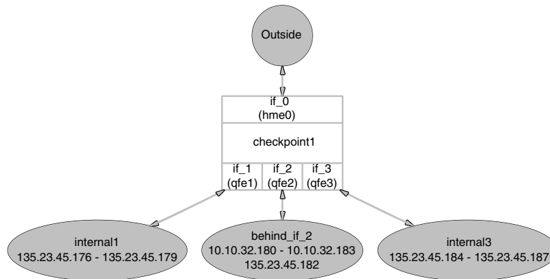
Fig. 10 A diagram of the firewall’s network connectivity, derived from the network topology description file
