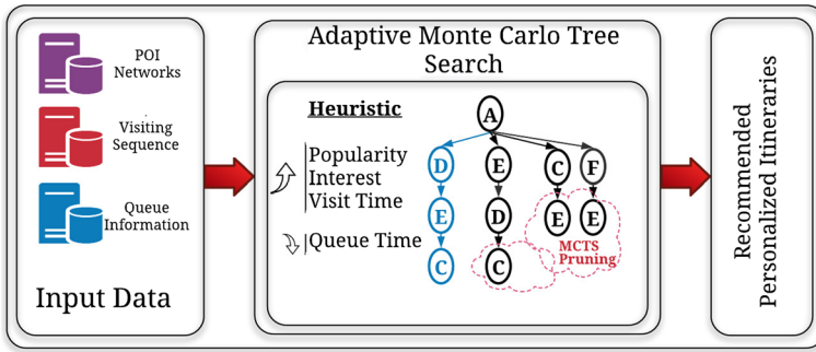
Fig. 3 Working steps of proposed EffiTourRec recommendation system
