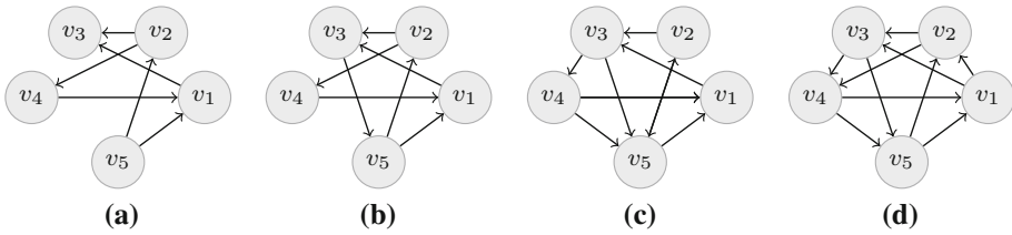
Fig. 1 Toy example showing an anonymization process from the original graph to an Independent 2-degree, Independent (1, 2)-degree and Paired 5-degree anonymous versions of the same network. a Original network, b Independent 2-anonymous, c Independent (1, 2)-anonymous, d paired 5-degree anonymous
