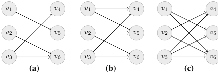
Fig. 3 Order for adding edges may be relevant. a Original graph, b adding (v_1, v_4) and (v_2, v_5) , c adding (v_1, v_6) , (v_2, v_4) and (v_3, v_5)
