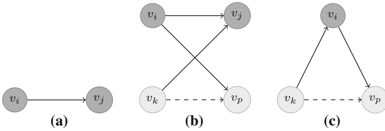
Fig. 2 Illustration of edge addition, switch and extension processes. Solid lines represent new edges to be added and dashed lines existing edges to be deleted. Vertex color indicates whether a vertex changes its degree (dark gray) or not (light gray) after the edge modification has been carried out. a Edge addition, b edge switch, c edge extension
