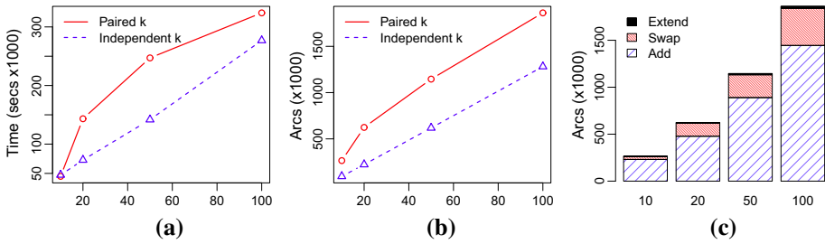
Fig. 7 Details of our experiments on Pokec network. The horizontal axis represents the k -degree anonymity value. a Computation time, b new arcs, c detail of new arcs
