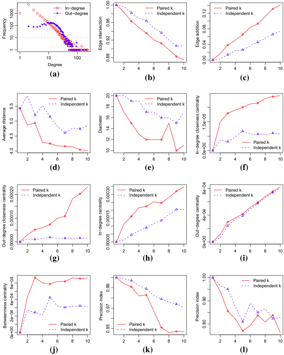
Fig. 5 Generic and clustering information loss evaluation on Paired k and Independent k -degree anonymity on DBLP-CITE dataset. a Degree distribution, b EI , c EA , d dist , e d , f in-degree C_C , g out-degree C_C , h in-degree C_D , i out-degree C_D , j C_B , k Infomap , l Walktrap
