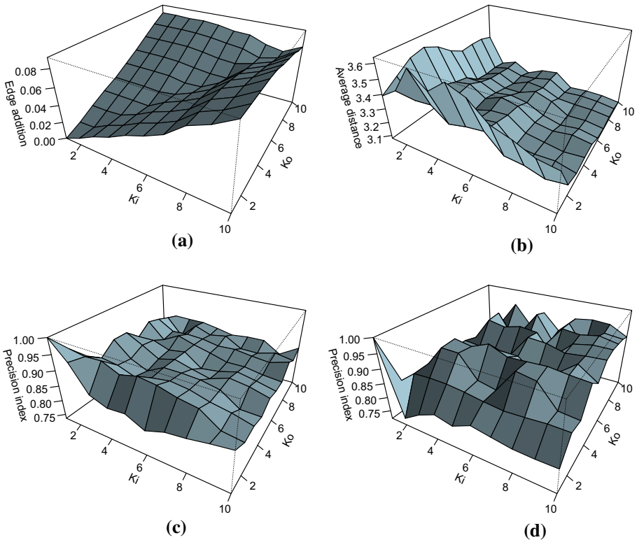
Fig. 6 Independent (k_i, k_o) -degree anonymity on POLBLOGS dataset. a Degree distribution, a EA, b \overline{dist} , c Infomap, d Walktrap
