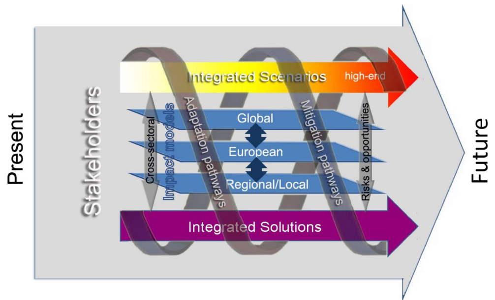
Fig. 1 Schematic of the overall IMPRESSIONS approach to co-creating integrated solutions to high-end climate change with stakeholders
