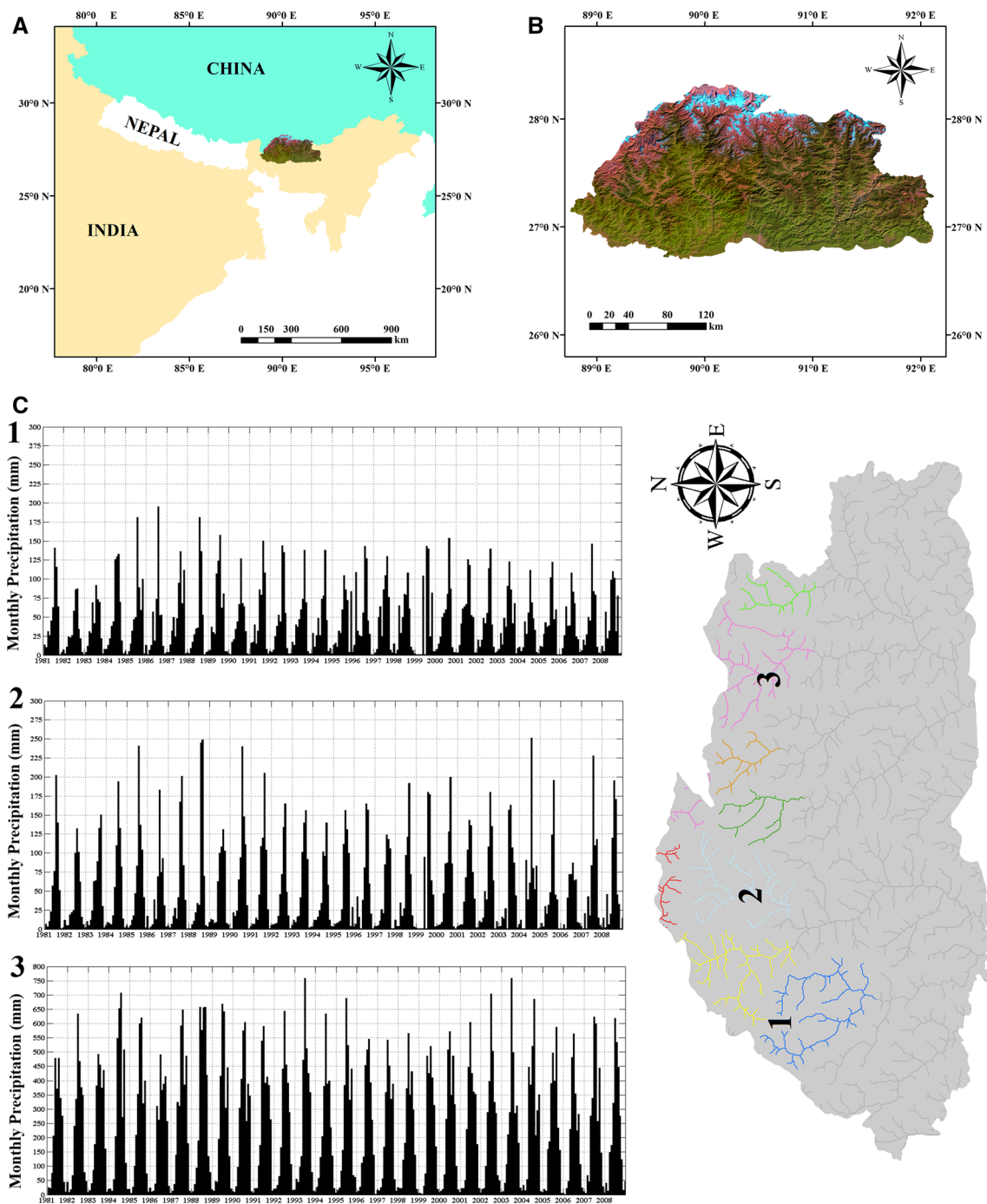
Fig. 1 a Geographical location of Bhutan. b Land cover of Bhutan (5-4-3 Landsat false-colour composite). c The west-to-east precipitation gradient in the Bhutan Himalaya
