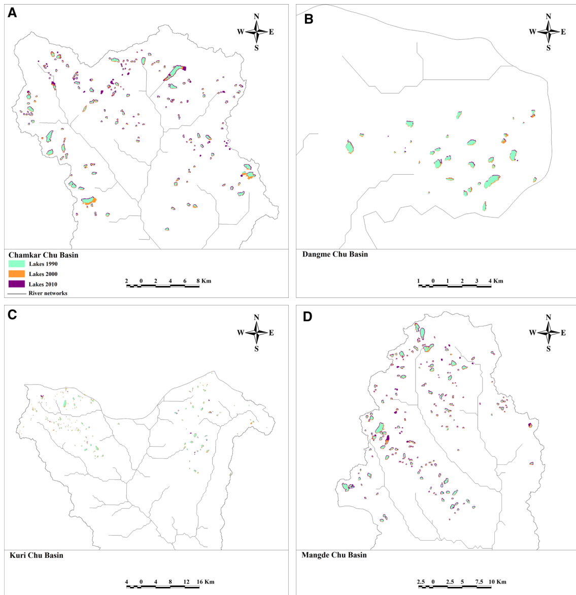
Fig. 5 Changes in glacial lakes in eight river basins (Chamkar Chu, Dangme Chu, Kuri Chu, Mangde Chu, Mo Chu, Northern Basin, Pho Chu and Wang Chu) in the Bhutan Himalaya (1990–2010)
