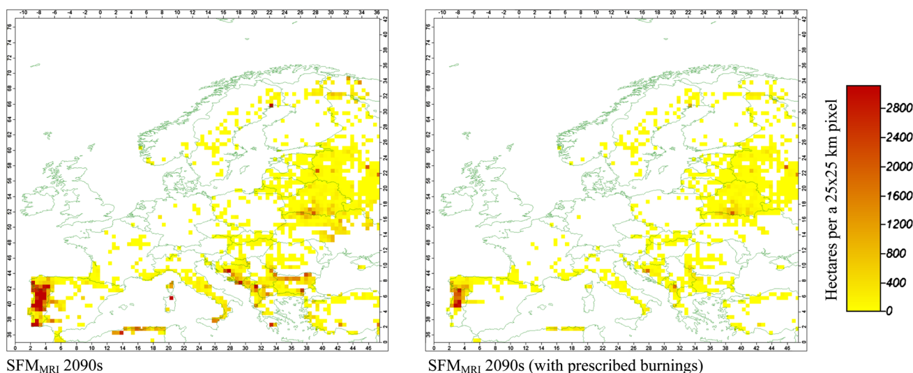
Fig. 3 Spatially, explicit projection of yearly burned areas (hectares per a 25 × 25 km pixel) estimated by SFM MRI model in 2090s with and without prescribed burnings
