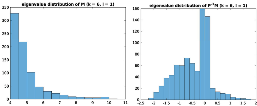
Fig. 1 Eigenvalue distribution of M and P^{-1}M at the first Newton’s iteration (last outer iteration)
