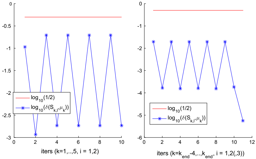
Fig. 4 Problem G11: Values of \delta(S_{k,\ell}, \mu_k) for \ell = 1, 2, (3) in first 5 (left figure) and last 5 (right figure) outer iterations (logarithmic scale)
