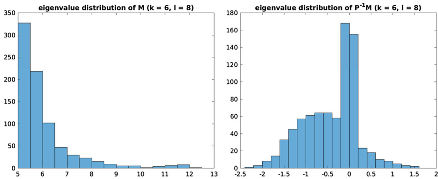
Fig. 2 Eigenvalue distribution of M_\ell and P^{-1}M_\ell at the last Newton’s iteration (last outer iteration)
