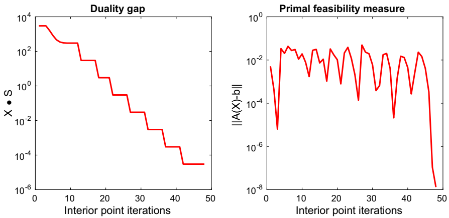
Fig. 3 Problem G48: duality gap and primal feasibility
