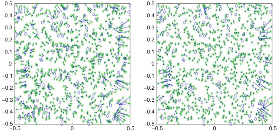
Fig. 4 The left figure shows the anchor (“o”) and the solution found by LPCGD for problem 4 in Table 1 ( n = 1,000, \sigma = 0.1 ). Each sensor position (“.”) found is joined to its true position (“*”) by a line . The right figure shows the same information for the solution found by LPCGD( m,I ) using Version B of local improvement
