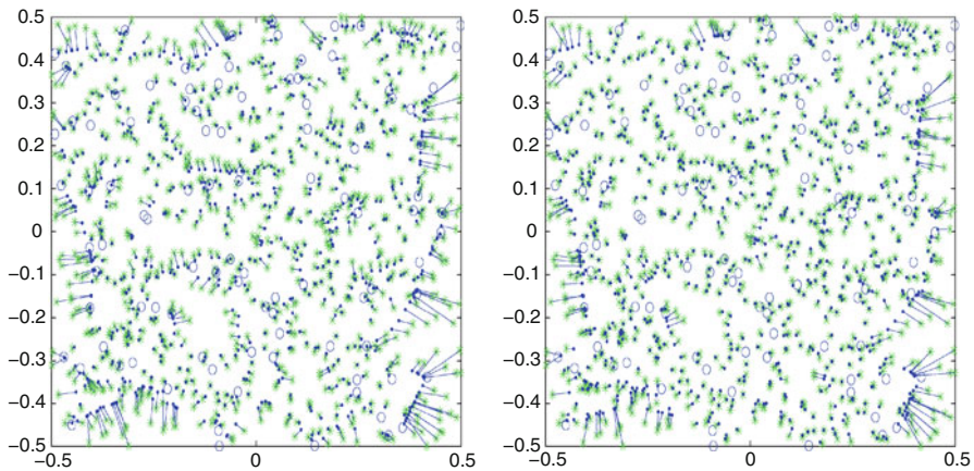
Fig. 3 The left figure shows the anchor (“o”) and the solution found by LPCGD for problem 4 in Table 1 ( n = 1,000, \sigma = 0.1 ). Each sensor position (“.”) found is joined to its true position (“*”) by a line. The right figure shows the same information for the solution of ESDP found by SeDuMi-I06 for the same problem
