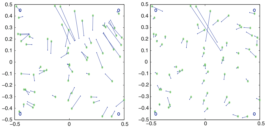
Fig. 6 The left figure shows the anchor (“o”) and the solution found by LPCGD for problem 2 in Table 7 ( m = 60, \sigma = 0.2 ). Each sensor position (“.”) found is joined to its true position (“*”) by a line. The right figure shows the same information for the solution found by LPCGD( m,I ) using Version B of local improvement
