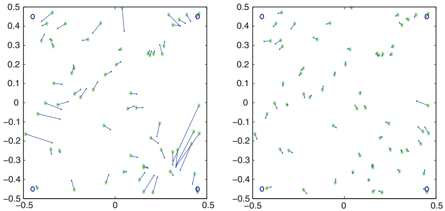
Fig. 5 The left figure shows the anchor (“o”) and the solution found by LPCGD for problem 1 in Table 7 ( m = 60, \sigma = 0.1 ). Each sensor position (“.”) found is joined to its true position (“*”) by a line . The right figure shows the same information for the solution found by LPCGD( m,I ) using Version B of local improvement
