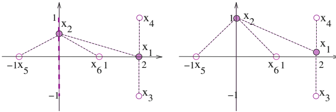
Fig. 1 An example showing that, when distance measurements have noise, zero individual trace is uninformative of sensor position accuracy in ESDP and SDP solutions
