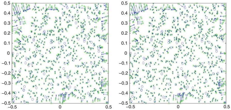
Fig. 2 The left figure shows the anchor (“o”) and the solution found by LPCGD for problem 3 in Table 1 ( n = 1,000, \sigma = 0.01 ). Each sensor position (“.”) found is joined to its true position (“*”) by a line. The right figure shows the same information for the solution of ESDP found by SeDuMi-106 for the same problem
