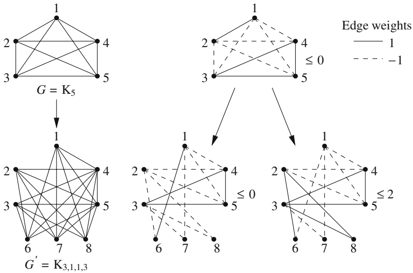
Fig. 1 A graph G' and two inequalities obtained as the triangular eliminations of G = K_5 and its facet inducing pentagonal inequality
