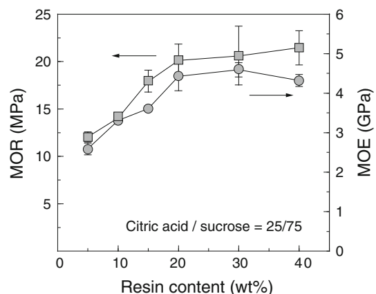
Fig. 6 Effect of resin content of citric acid/sucrose on bending properties. Error bars indicate standard deviations
