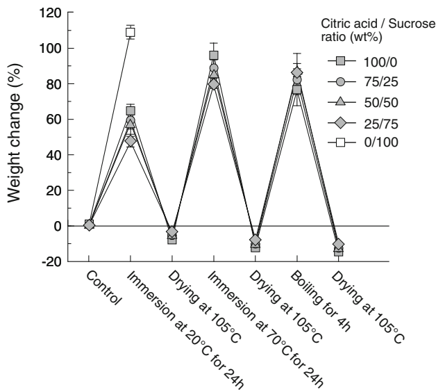
Fig. 5 Weight change in a cyclic accelerated aging treatment. Error bars indicate standard deviations
