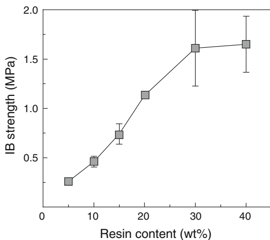
Fig. 7 Effect of resin content of citric acid/sucrose on IB strength. Error bars indicate standard deviations
