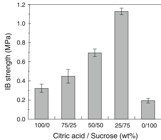
Fig. 3 Effect of citric acid/sucrose ratio on IB strength. Error bars indicate standard deviations
