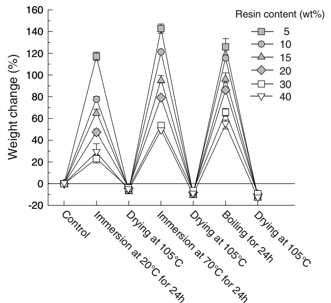
Fig. 9 Weight change in a cyclic accelerated aging treatment. Error bars indicate standard deviations
