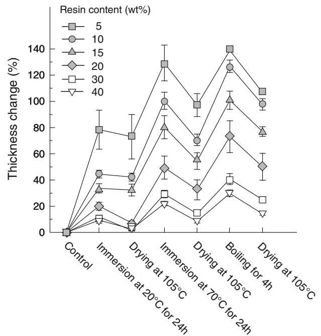
Fig. 8 Thickness change in a cyclic accelerated aging treatment. Error bars indicate standard deviations
