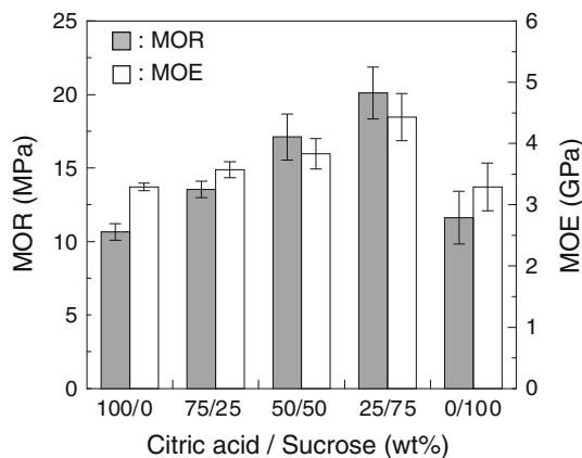
Fig. 2 Effect of citric acid/sucrose ratio on bending properties. Error bars indicate standard deviations
