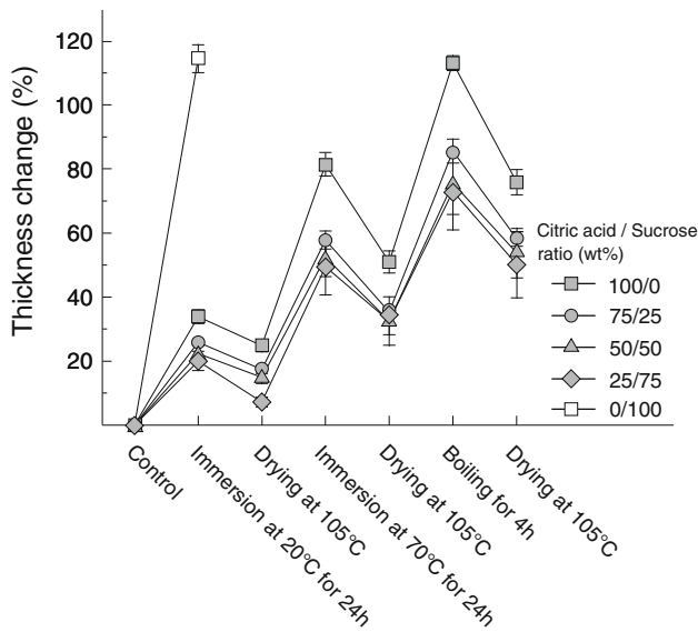
Fig. 4 Thickness change in a cyclic accelerated aging treatment. Error bars indicate standard deviations
