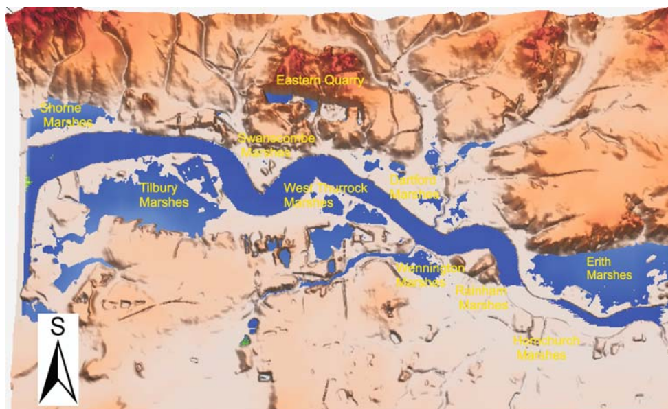
Fig. 12 Intersection of simulated groundwater table for February 1995 (blue) with DTM within the West Thurrock area
