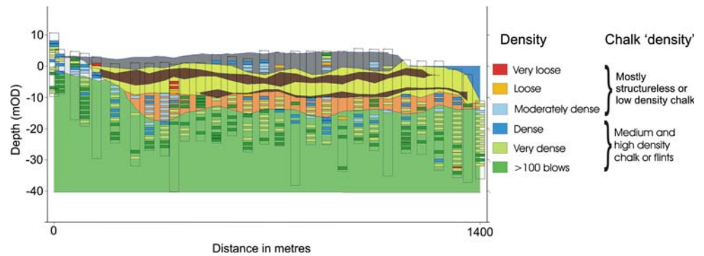
Fig. 8 Cross-section showing the variation of SPT values within the Thames Gravels and Chalk within grid square TQ57NW
