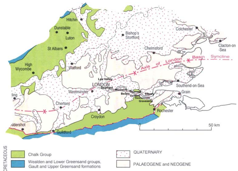
Fig. 1 Geological map of London and the surrounding area
