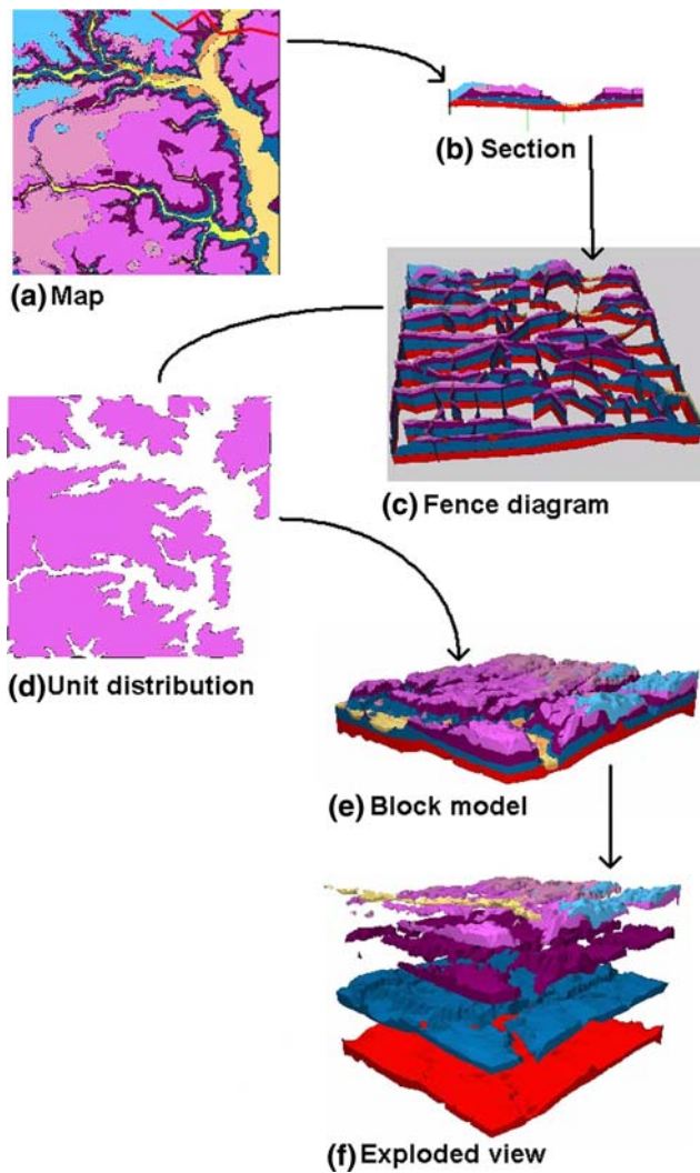
Fig. 3 3D geological model building work flow in GIS3D (after Kessler and Mathers 2004)
