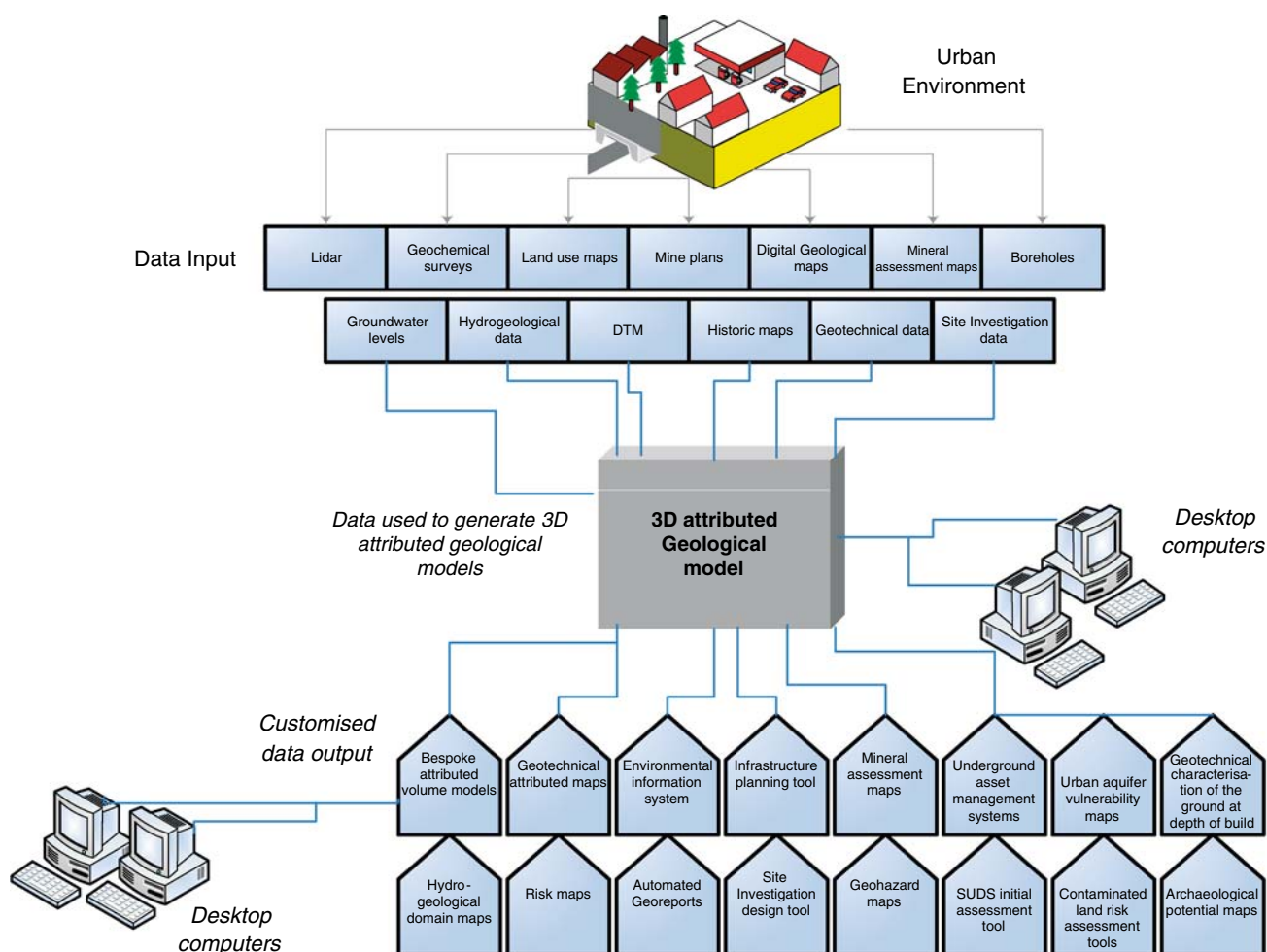
Fig. 2 Flow diagram showing the process of building and applications of the 3D attributed geological model
