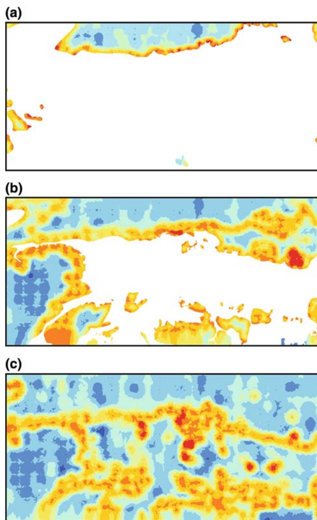
Fig. 13 Grids displaying confidence data in the Thames Gateway region between Woolwich and Gravesend for a London Clay formation, b Thanet Sand formation and c the Chalk Group. Colour variation from blue to red indicates a change from low to high confidence
