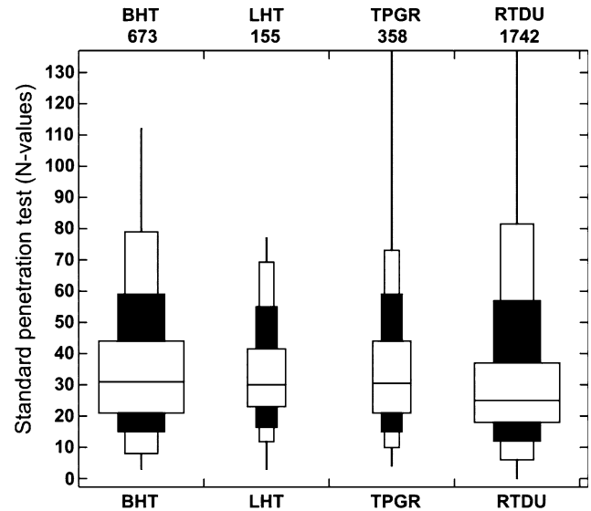
Fig. 4 Box and whisker plot of standard penetration test results for the terrace gravels in part of the Thames Gateway area. BHT Boyne Hill gravel formation, LHT Lynch Hill gravel formation, TPGR Taplow gravel formation and RTDU Kempton Park and Shepperton gravel formations
