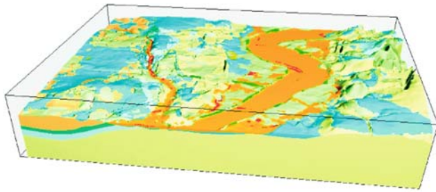
Fig. 5 3D block model of the engineering geological classification of the area between Dartford and Thurrock (see Table 1 for key)
