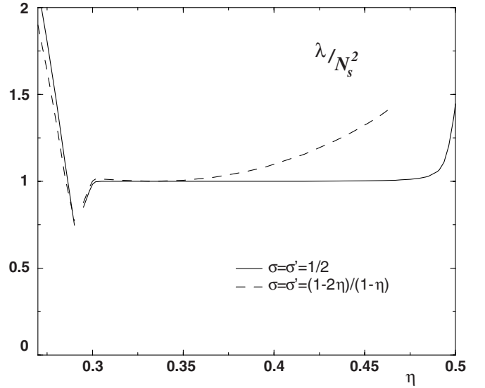
Fig. 4. Dependence of \lambda/N_s^2 on \eta for fixed \sigma = \sigma' = 1/2 (solid) and with \sigma, \sigma' from eq. (3.13) (dashed). The width \gamma_2 is fixed to yield \lambda/N_s^2 = 1 at \eta = 1/3 .
