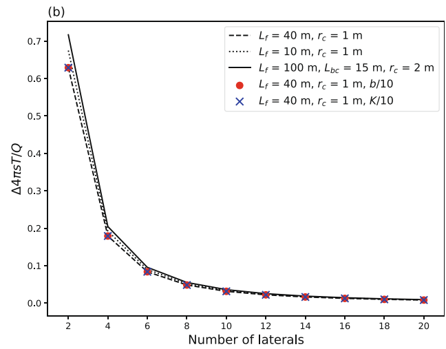
dimensionless drawdown between Hantush and Papadopoulos (1962) and Theis (1935) equations at the tip of the lateral for different numbers of laterals. Parameters are listed in Table 3
