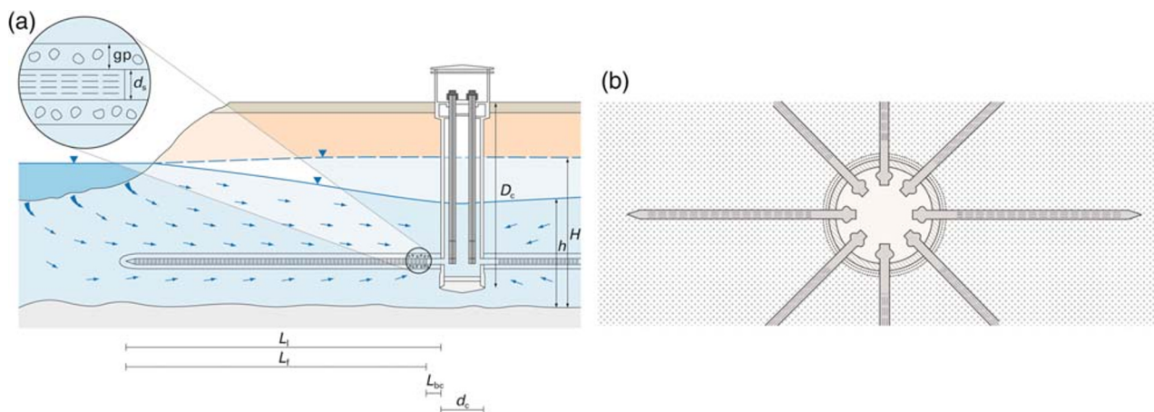
Fig. 1 a Cross-section and b plan view of a radial collector well. L_l , L_f , L_{bc} are total, screened and closed lateral length, respectively; d_c diameter of the caisson; D_c caisson depth; gp gravel pack thickness; d_s diameter of lateral; H static head; h pumped head (©BGR)
