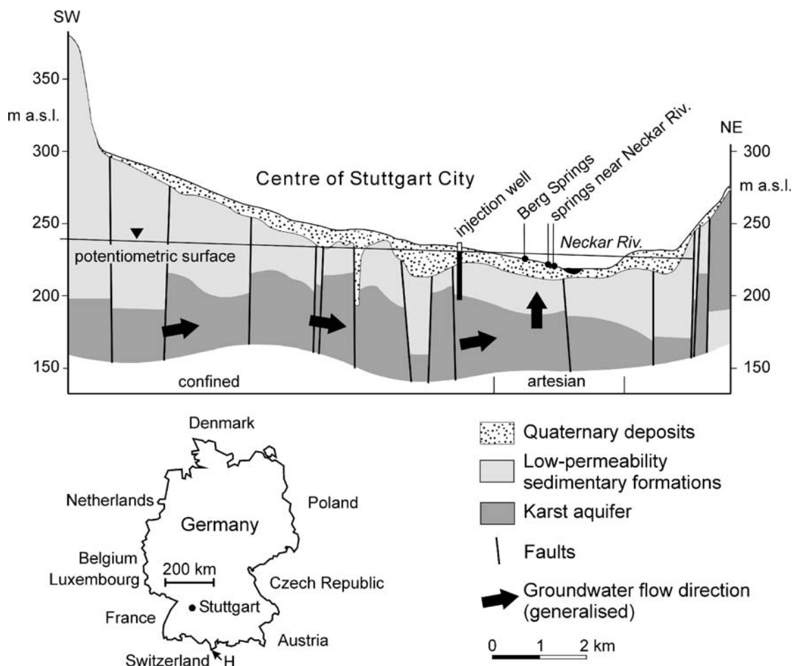
Fig. 1 Hydrogeological section of the artesian karst aquifer below the city of Stuttgart. The section cuts through the injection well and the two groups of mineral springs where the tracer breakthrough curves discussed in this article were observed. Z -axis strongly exaggerated (modified after Goldscheider et al. 2003). The location of the Hölloch cave ( H ) is also shown because data from there are presented for comparison
