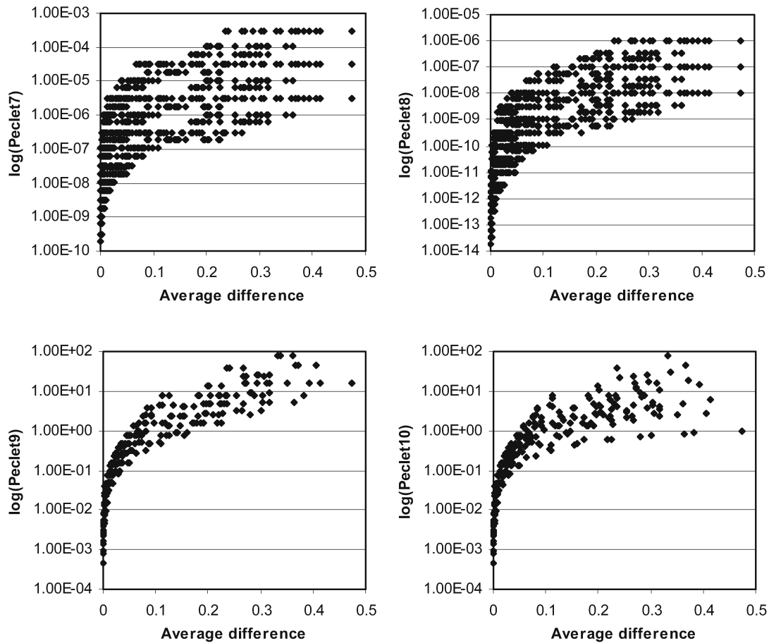
Figure 6 Relation between Péclet numbers 7 to 10 and the averaged difference between C/C_0 due to diffusion, advection and dispersion and C/C_0 due to diffusion only.
