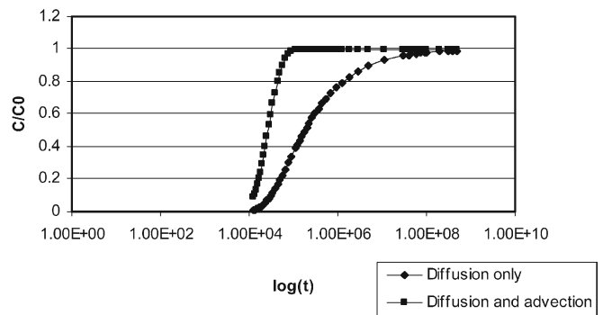
Figure 4 Concentration versus time for K=10^{-10} m/s, grad h=0.02 , n_e=0.001 , L=10 m, D_e=6 \cdot 10^{-4} m 2 /year, \alpha=0.01 m, resulting difference=30%
