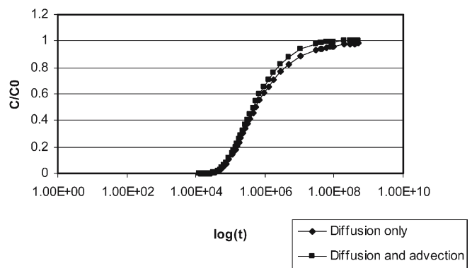
Figure 3 Concentration versus time for K=10^{-12} m/s, grad h=0.02 , n_e=0.001 , n=0.2 , L=10 m, D_e=2.05 \cdot 10^{-4} m 2 /year, \alpha=0.01 m; resulting difference=2%
