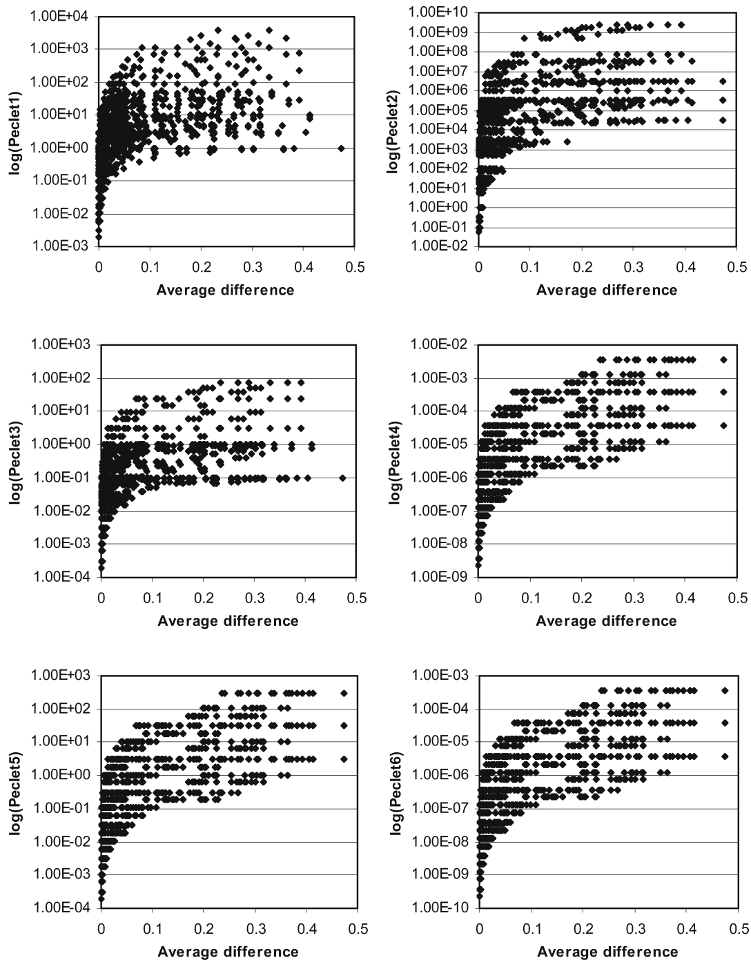
Figure 5 Relation between Péclet numbers 1 to 6 and the averaged difference between C/C_0 due to diffusion, advection and dispersion and C/C_0 due to diffusion only.
