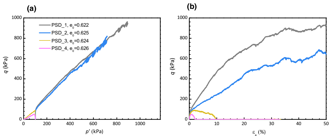
Fig. 6 Effects of PSD on constant volume shear behavior of samples with clumped particles ( OR=0.914 ) at p_0' = 100 kPa: a effective stress paths; b deviatoric stress–axial strain curves
