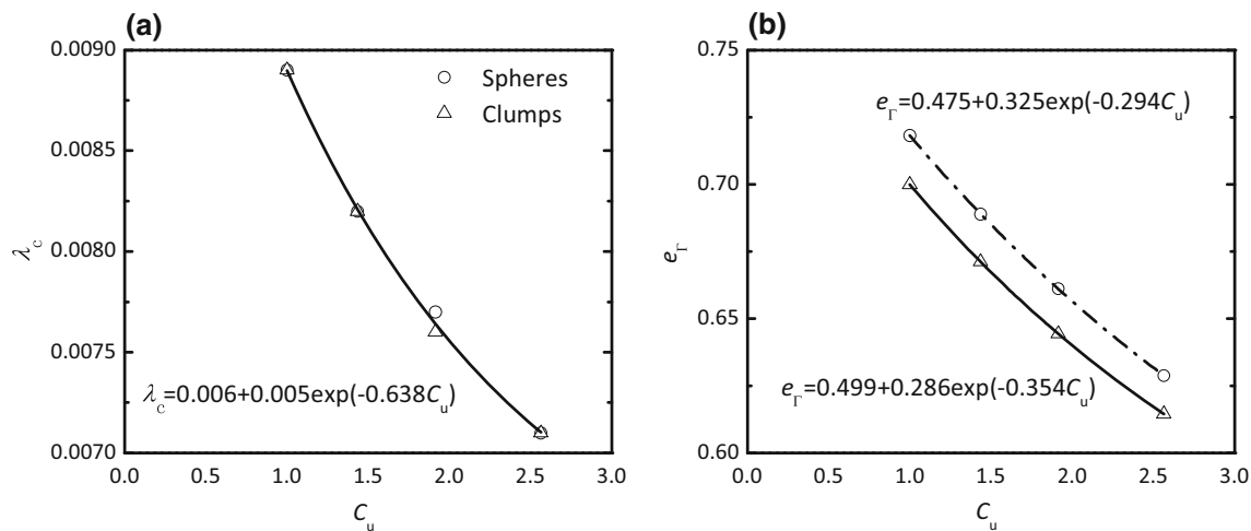
Fig. 15 Relationship between CSL parameters and C_u : a \lambda_c versus C_u ; b e_\Gamma versus C_u
