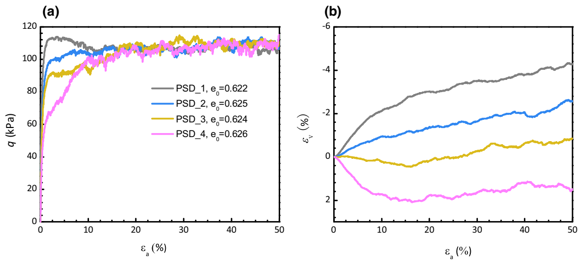
Fig. 7 Effects of PSD on constant p' shear behavior of samples with clumped particles ( OR=0.914 ) at p_0' = 100 kPa: a deviatoric stress–axial strain curves; b volumetric strain–axial strain relations
