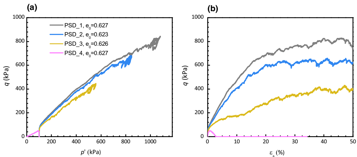
Fig. 4 Effects of PSD on constant volume shear behavior of samples with spherical particles ( OR=1 ) at p_0' = 100 kPa: a effective stress paths; b deviatoric stress–axial strain curves
