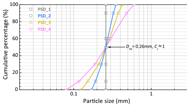
Fig. 3 Particle size distribution of assemblages
