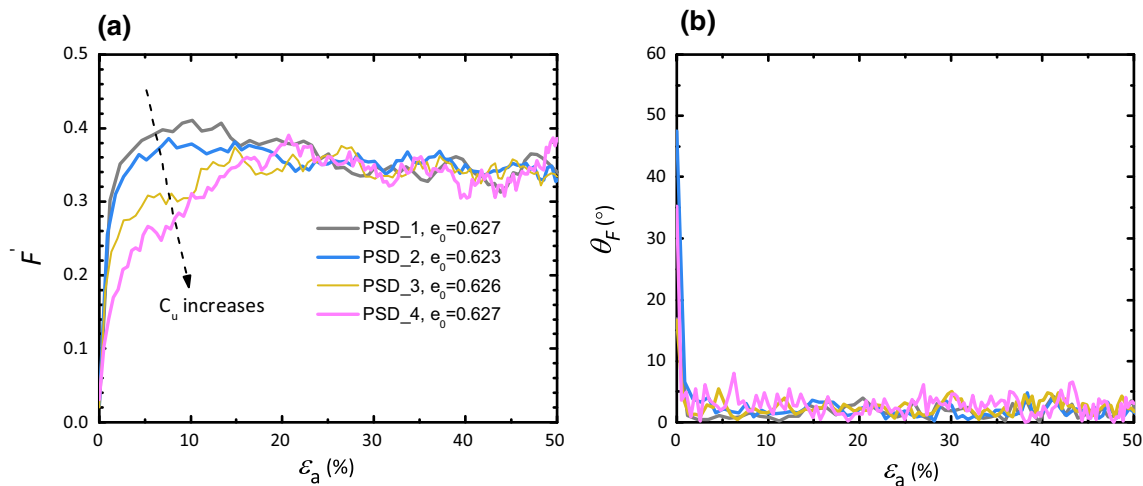
Fig. 8 Effects of PSD on the fabric evolution of samples with spherical particles ( OR=1 ) under constant p' test at p_0' = 100 kPa: a fabric norm F' ; b fabric Lode angle \theta_F
