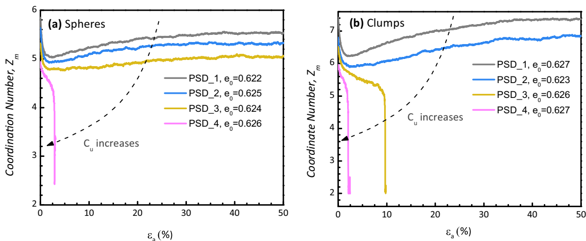
Fig. 11 Effects of PSD on the coordinate number under constant volume test at p_0' = 100 kPa: a spherical particles ( OR=1 ); b clumped particles ( OR=0.914 )
