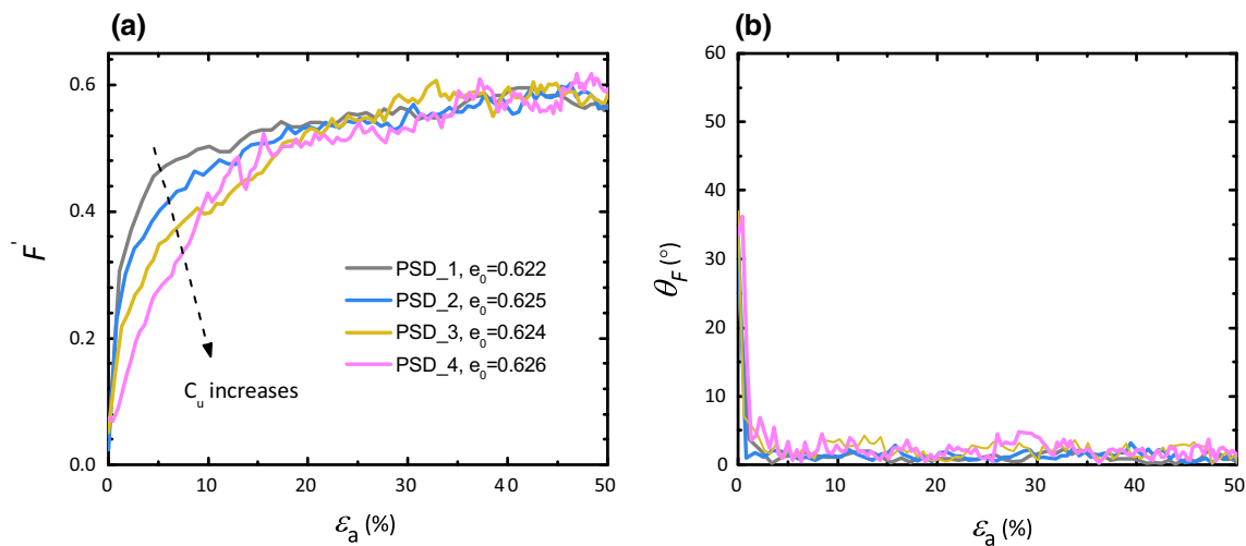
Fig. 9 Effects of PSD on the fabric evolution of samples with clumped particles ( OR=0.914 ) under constant p' test at p_0' = 100 kPa: a fabric norm F_c' ; b fabric Lode angle \theta_F
