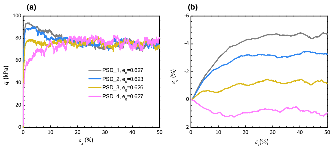
Fig. 5 Effects of PSD on constant p' drained shear behavior of samples with spherical particles ( OR=1 ) at p_0' = 100 kPa: a deviatoric stress–axial strain curves; b volumetric strain–axial strain relations
