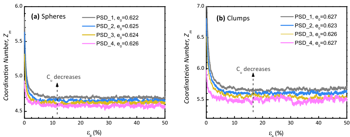
Fig. 10 Effects of PSD on the coordinate number under constant p' test at p_0' = 100 kPa: a spherical particles ( OR=1 ); b clumped particles ( OR=0.914 )
