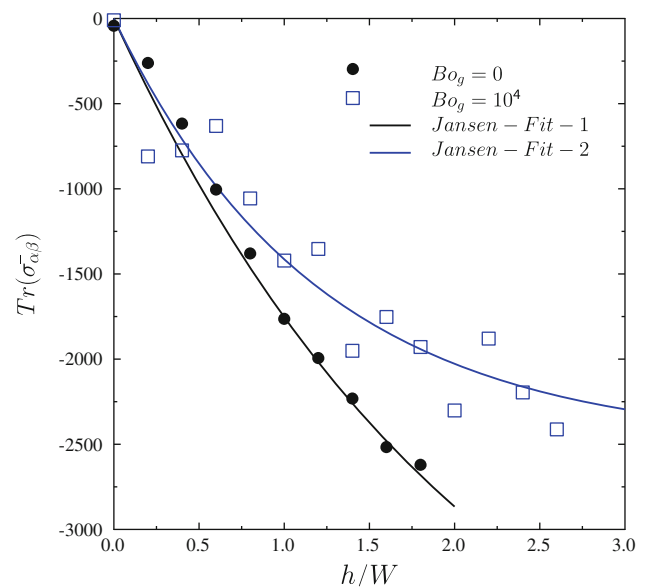
Fig. 5 Profiles of the trace of the mean stress tensor, obtained for particles with d = 10 and two different Bond numbers. The depth is normalized with the width W of the system. We also show the fitting to the equation \sigma = \sigma_m(1 - \exp(-x/h_s)) , where we used [ \sigma_m = 2,500 N/m; h_s/W = 1.2 ] and [ \sigma_m = 4,800 N/m; h_s/W = 2.2 ] for case 1 and 2, respectively
