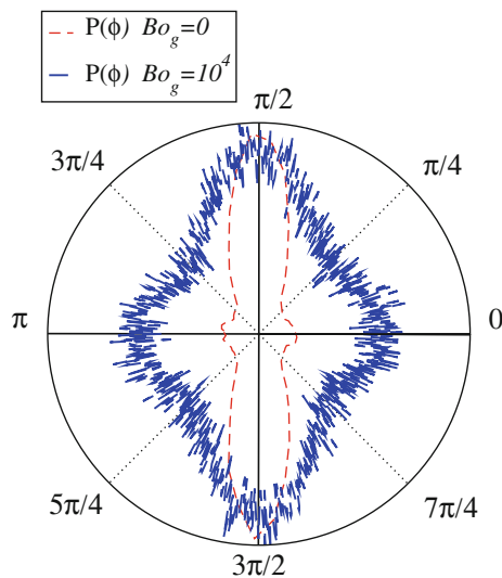
Fig. 4 (Color online) Polar distribution of the principal direction (larger eigenvalue of the stress tensor for each particle \sigma_{\alpha\beta} ), obtained for particles with d = 10 . For comparison, the data for Bo_g = 0 and Bo_g = 10^4 is presented
