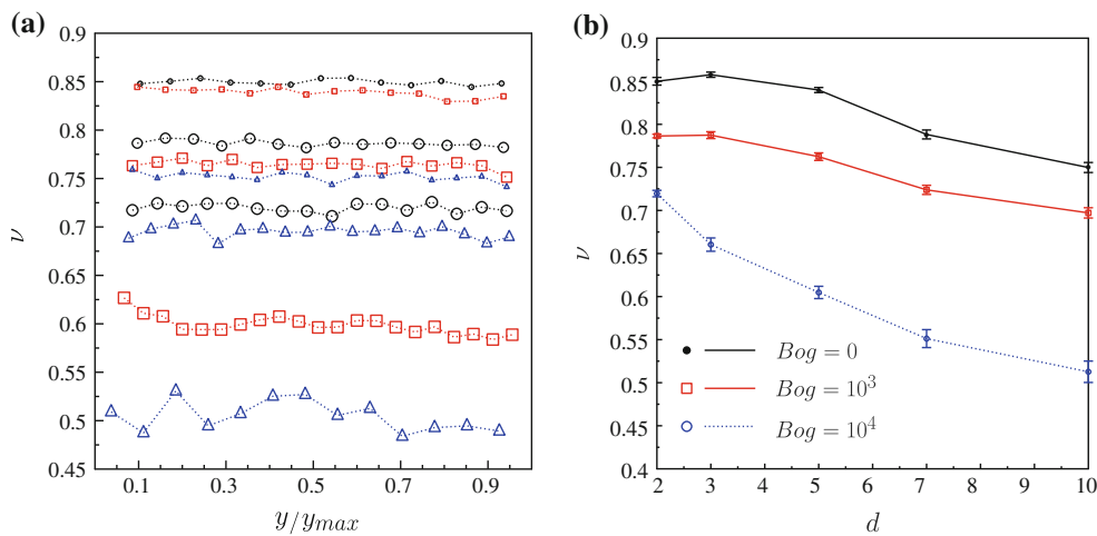
Fig. 2 (Color online) Density profiles of different granular deposits. In a the circles represent particles with d = 2 , the squares d = 5 and the triangles d = 10 . The larger the symbols the stronger is the attractive
