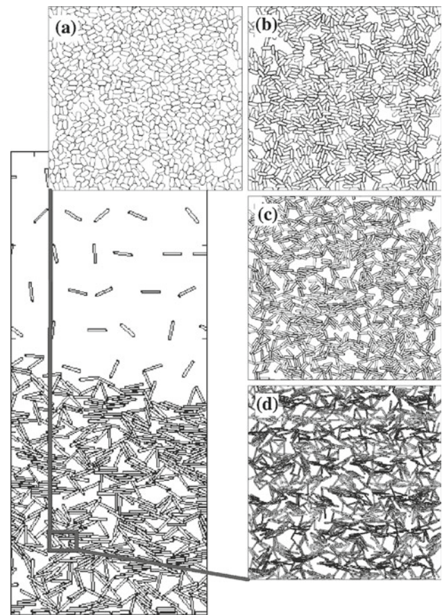
Fig. 1 Simulated packings of elongated cohesive particles settled by gravity. Final configurations are shown for the same granular Bond number Bo_g = 10^3 and increasing elongation: a d = 2 , b d = 3 , c d = 5 and d d = 10
