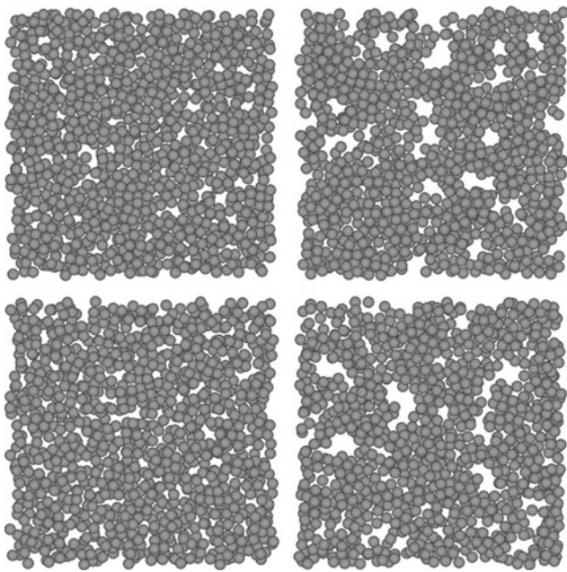
Fig. 1 Slices through VEM-microstructures (upper row) with a more homogeneous microstructure ( N_V = 16,000 , left) and a more heterogeneous microstructure ( N_V = 1,000 , right). The lower row shows the most homogeneous ( \Psi_0 = 0 mV, left) and most heterogeneous microstructure ( \Psi_0 = 15 mV, right) resulting from earlier BD-simulations [26]. Slice thickness: three particle diameters; particle diameter = 0.5 \mu\text{m} , volume fraction = 0.4 (for all structures)
