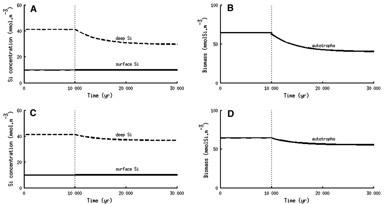
Figure 4. Regulation of silicic acid concentrations in the ocean. Nutrient supply is decreased by 50% after a third of the simulation time (dotted vertical line). Simulations are performed from the application of the generic model to the oceanic cycle of silicic acid with realistic parameter values. Bold lines and dotted lines are for the surface and deep silicic acid pools, respectively. A Regulation of silicic acid concentrations in case of a decrease in the supply of surface silicic acid ( \rho = 1 and \rho = 0.44 for the accessible and inaccessible pools, respectively). B Impact of a decrease in the supply of surface silicic acid on the biomass of autotrophic organisms. C Regulation of silicic acid concentrations in case of a decrease in the supply of surface silicic acid ( \rho = 1 and \rho = 0.78 for the accessible and inaccessible pools, respectively). D Impact of a decrease in the supply of deep silicic acid on the biomass of autotrophic organisms.
