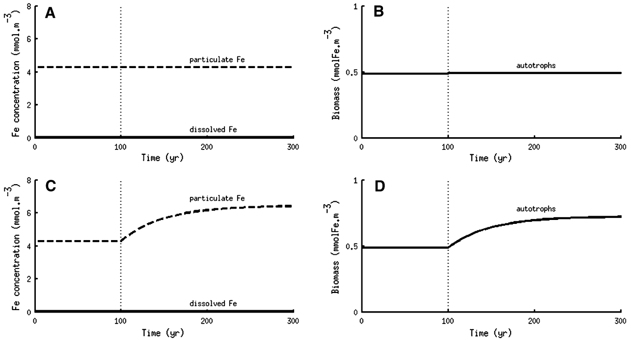
Figure 3. Regulation of iron concentrations in the ocean. Nutrient supply is increased by 50% after a third of the simulation time ( dotted vertical line ). Simulations are performed from the application of the generic model to the oceanic cycle of iron with realistic parameter values. Bold lines and dotted lines are for the dissolved and particulate iron pools, respectively. A Regulation of iron concentrations in case of an increase in the supply of dissolved iron ( \rho = 1 for both pools). B Impact of an increase in the supply of dissolved iron on the biomass of autotrophic organisms. C Regulation of iron concentrations in case of an increase in the supply of particulate iron ( \rho = 1 and \rho = 2.3 \times 10^{-3} for the dissolved and particulate pools, respectively). D Impact of an increase in the supply of particulate iron on the biomass of autotrophic organisms.
