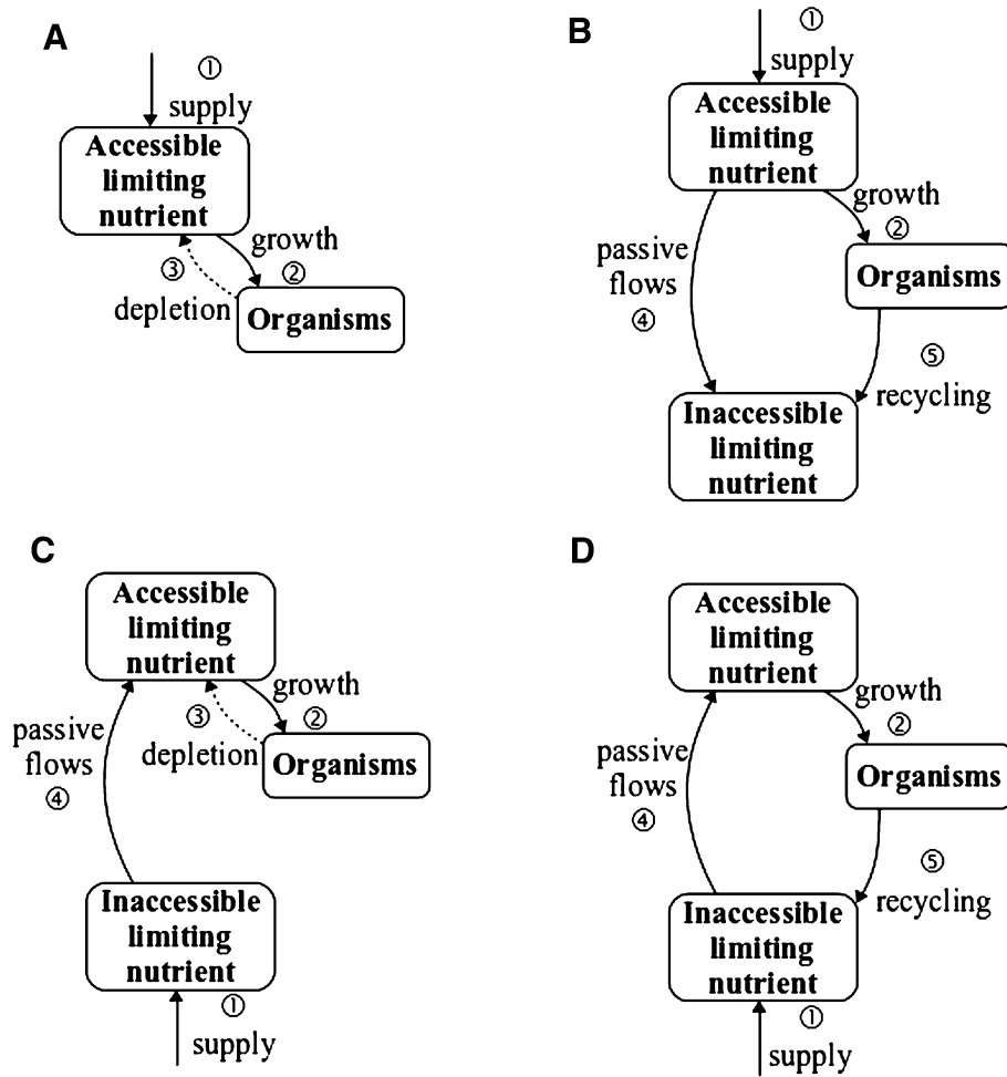
Figure 2. Regulation processes in the generic model. A Impact of the supply of a limiting nutrient in accessible form on its concentration in the accessible pool. B Impact of the supply of a limiting nutrient in accessible form on its concentration in the inaccessible pool. C Impact of the supply of a limiting nutrient in inaccessible form on its concentration in the accessible pool. D Impact of the supply of a limiting nutrient in inaccessible form on its concentration in the inaccessible pool. Bold arrows indicate a direct relationship (for example, an increase in the concentration of the accessible limiting nutrient results in an increase in biomass). Dashed arrows indicate an inverse relationship (for example, an increase in biomass results in a decrease in nutrient concentration in the accessible pool).
