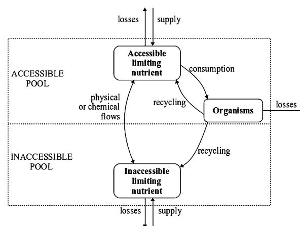
Figure 1. Generic model of nutrient dynamics with resource access limitation. Boxes and arrows represent stocks and flows, respectively.
