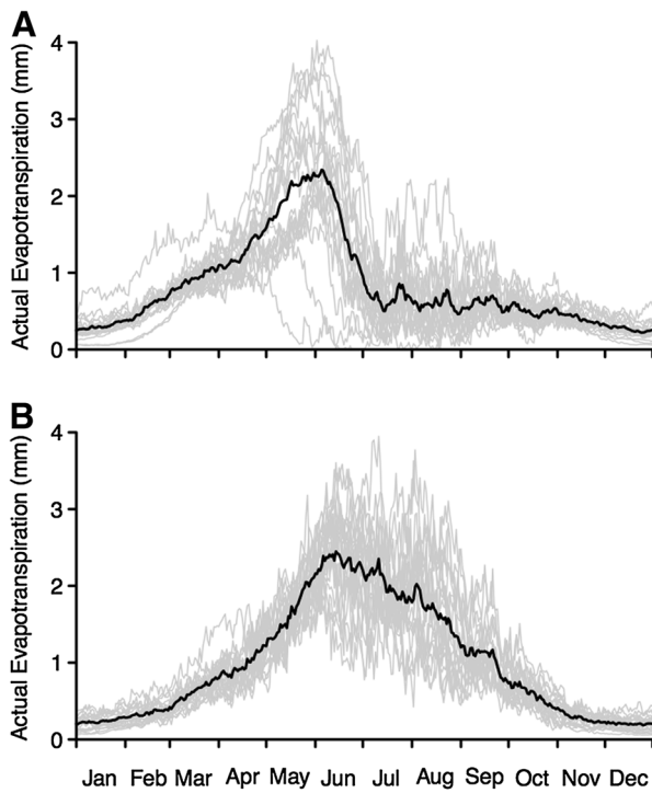
Figure 6. Long-term (30 years) simulated mean daily actual evapotranspiration for 20 Intermountain sites (A) and 20 Great Plains sites (B). The bold black lines are the means of the sites.
