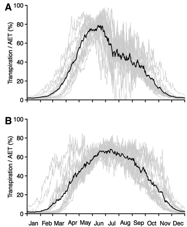
Figure 7. Long-term (30 years) simulated mean daily transpiration/actual evapotranspiration for 20 Intermountain sites (A) and 20 Great Plains sites (B). The bold black lines are the means of the sites.
