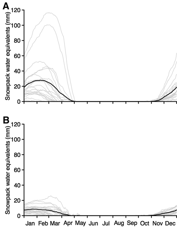
Figure 2. Long-term (30 years) simulated mean daily snow water equivalent in the snowpack for 20 Intermountain sites (A) and 20 Great Plains sites (B). The bold black lines are the means of the sites.
