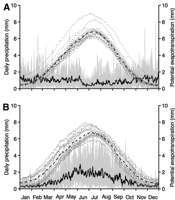
Figure 1. Long-term (30 year) mean daily precipitation and potential evapotranspiration for 20 Intermountain sites (A) and 20 Great Plains sites (B). The bold black lines are the means of the sites.
