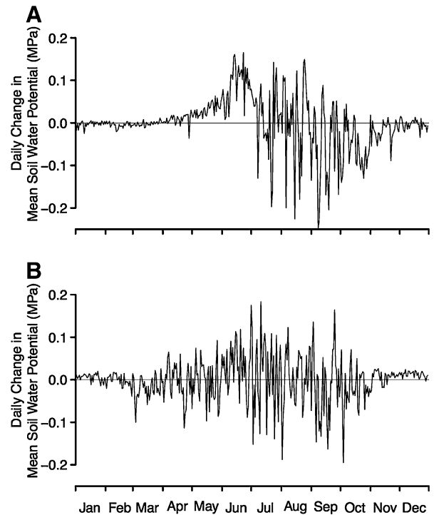
Figure 5. Long-term (30 years) mean daily changes in simulated soil water potential for the 0–30 cm layer for the mean of 20 Intermountain sites (A) and the mean of 20 Great Plains sites (B).
