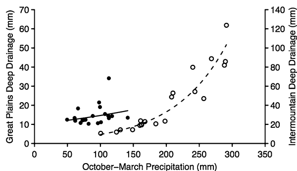
Figure 8. Regression relationships between long-term (30 years) simulated mean daily deep drainage and October–March precipitation for 20 Intermountain sites (dotted line and white points; r^2 = 0.92 ) and 20 Great Plains sites (continuous line and black points; r^2 = 0.10 ).
