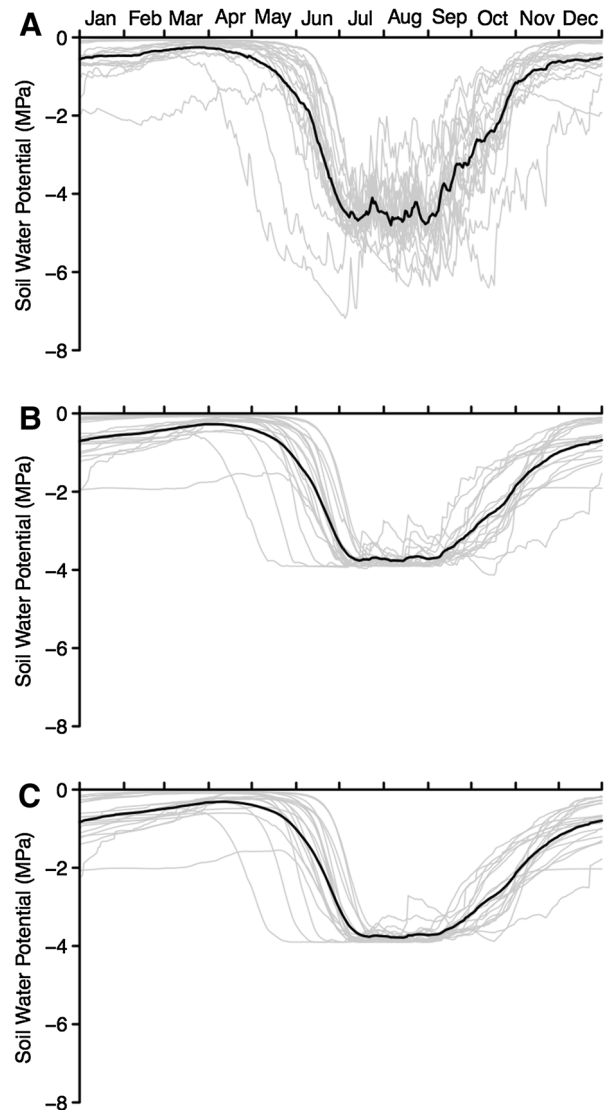
Figure 3. Long-term (30 years) simulated mean daily soil water potential in the 0-30 cm layer (A), 30-60 cm layer (B), and 60-100 cm layer (C) for 20 Intermountain sites. The bold black lines are the means of the sites.
