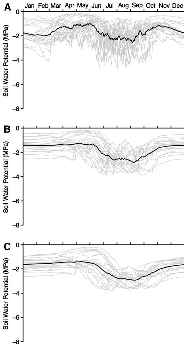
Figure 4. Long-term (30 years) simulated mean daily soil water potential in the 0–30 cm layer (A), 30–60 cm layer (B), and 60–100 cm layer (C) for 20 Great Plains sites. The bold black lines are the means of the sites.
