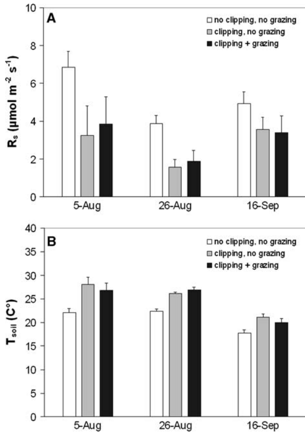
Figure 5. Effects of clipping and grazing on A soil \text{CO}_2 efflux and B soil temperature at Amplerio during the summer of 2004 (for each treatment n = 9 ).
