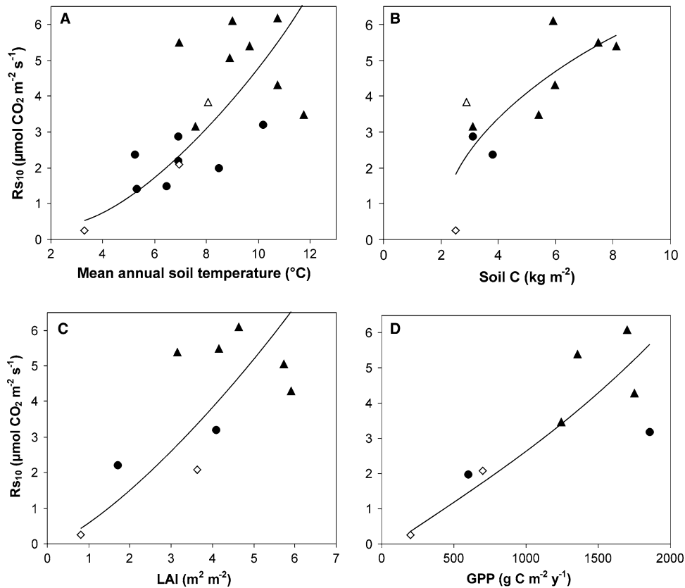
Figure 1. Soil respiration at a reference temperature (10°C) in relation to A mean annual soil temperature ( r^2 = 0.69 , P < 0.001 ), B soil C content in the uppermost 20–25 cm of the soil ( r^2 = 0.50 , P < 0.05 ), C peak leaf area index ( r^2 = 0.55 , P < 0.01 ) and D annual gross primary productivity ( r^2 = 0.88 , P = 0.001 ). Meadows (▲), pastures (●), unmanaged Northern grasslands (◇).
