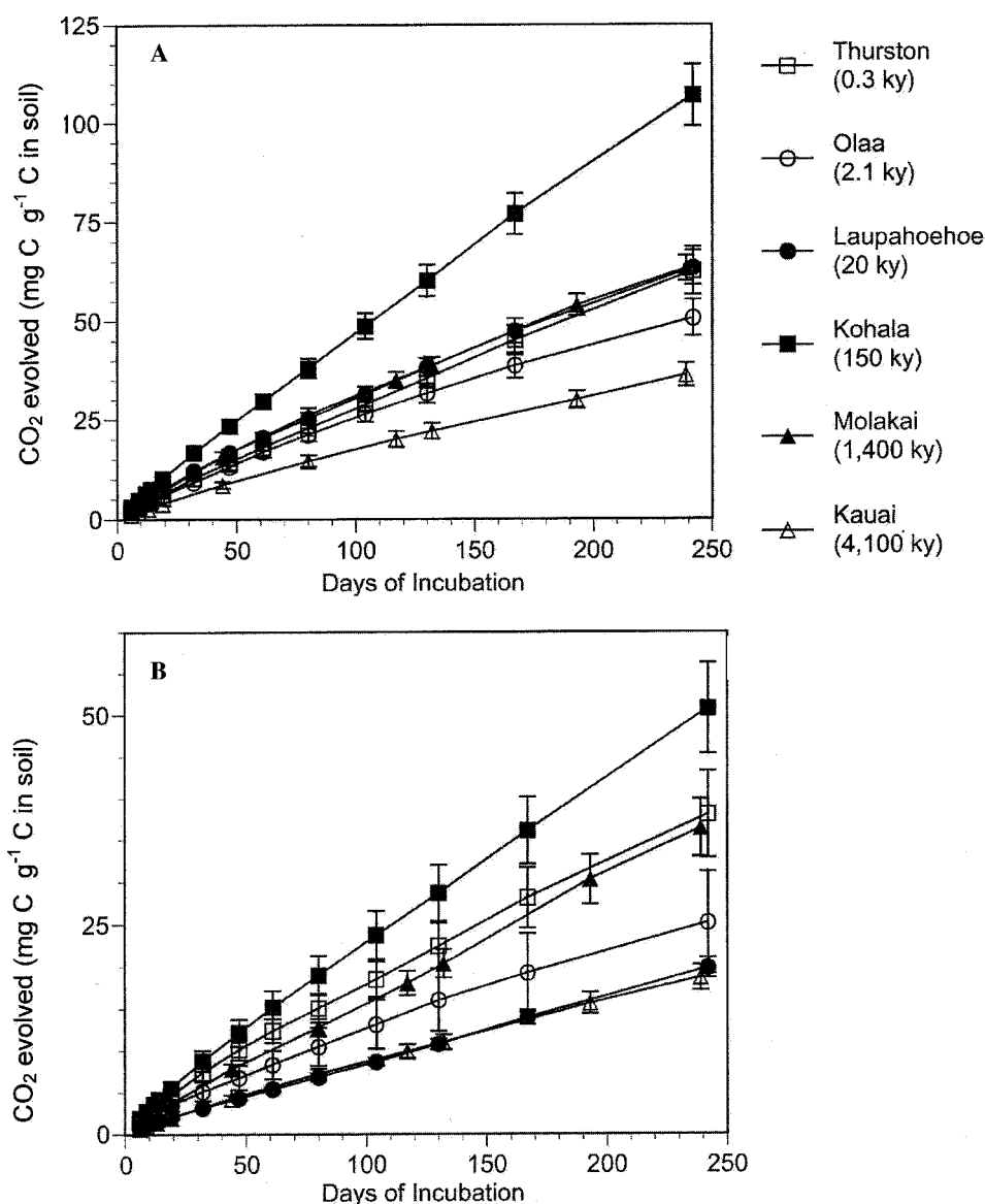
Figure 1. Cumulative \text{CO}_2 evolution from soils of the (a) O horizon and (b) A horizon. Error bars are \pm 1 standard error, n = 10 . Differences in emissions ( \text{g C} emitted per \text{g soil C} ) reflect differences in decomposability rather than in amount of organic carbon. In both horizons, the 150 ky site had greater cumulative respiration than the other sites and the oldest site had the lowest respiration rate. At each site, the A horizon had lower emission rates than the O horizon.
