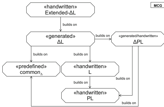
Fig. 4 Language hierarchy of concrete delta languages extended by PL and ΔPL
