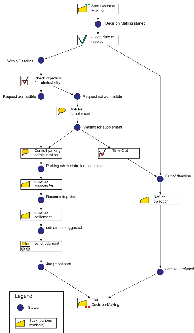
Fig. 1 An example decision-making process about objections against parking fines, modelled in Protos
