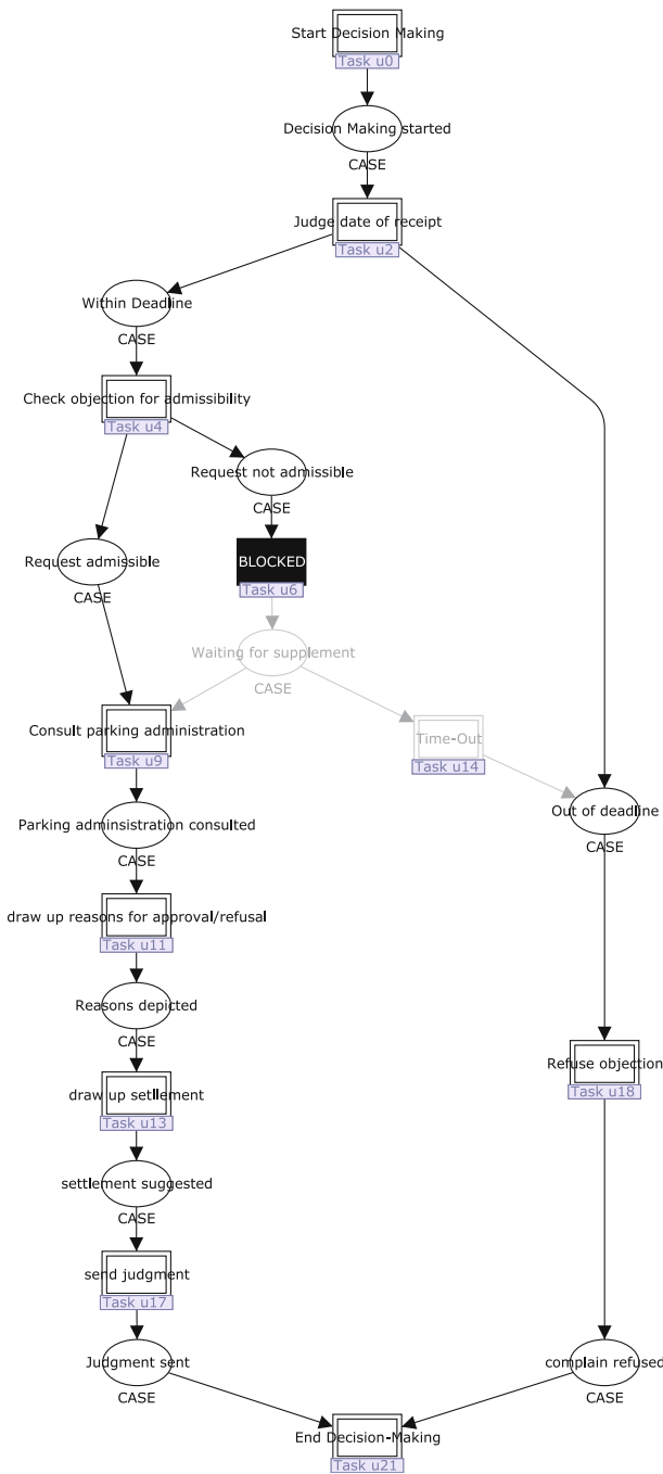
Fig. 14 Task Ask for supplement blocked (black): lost tokens may remain in the place Request not admissible
