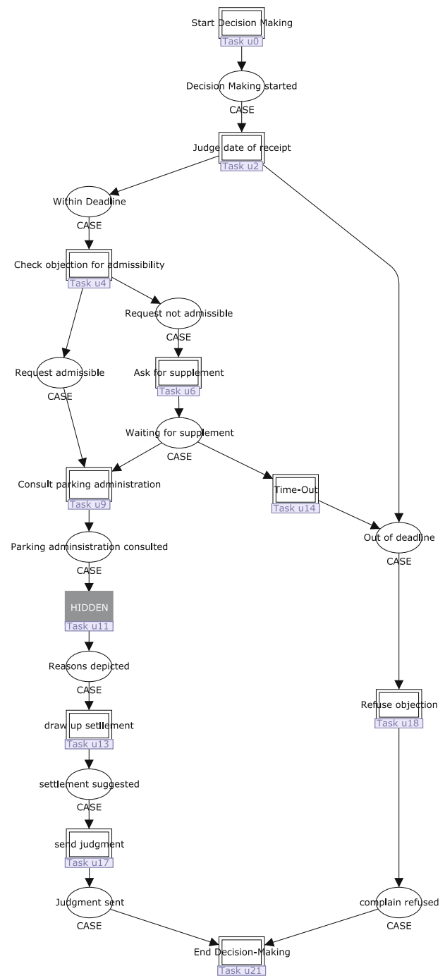
Fig. 10 Task draw up reasons for approval/refusal hidden (grey)
