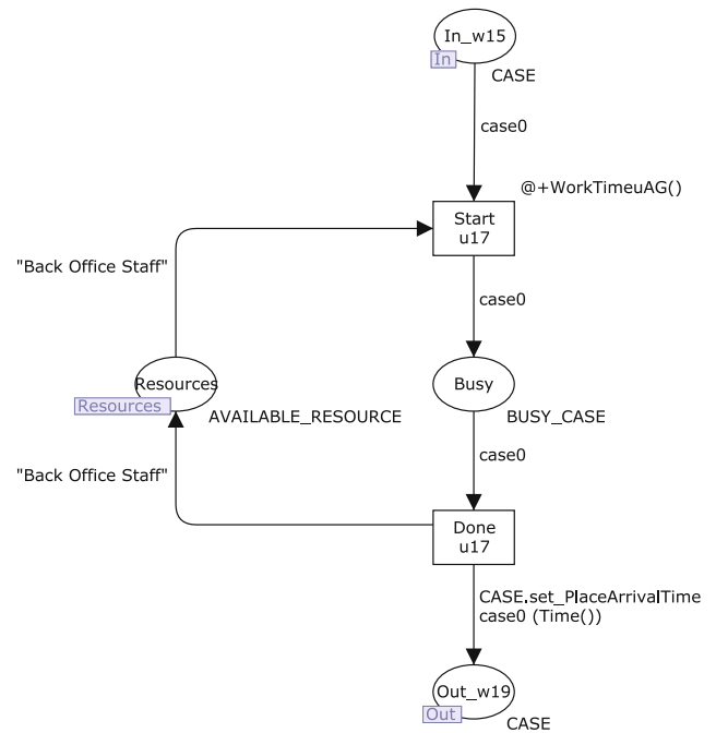
Fig. 3 Dedicated task page with information for simulation
