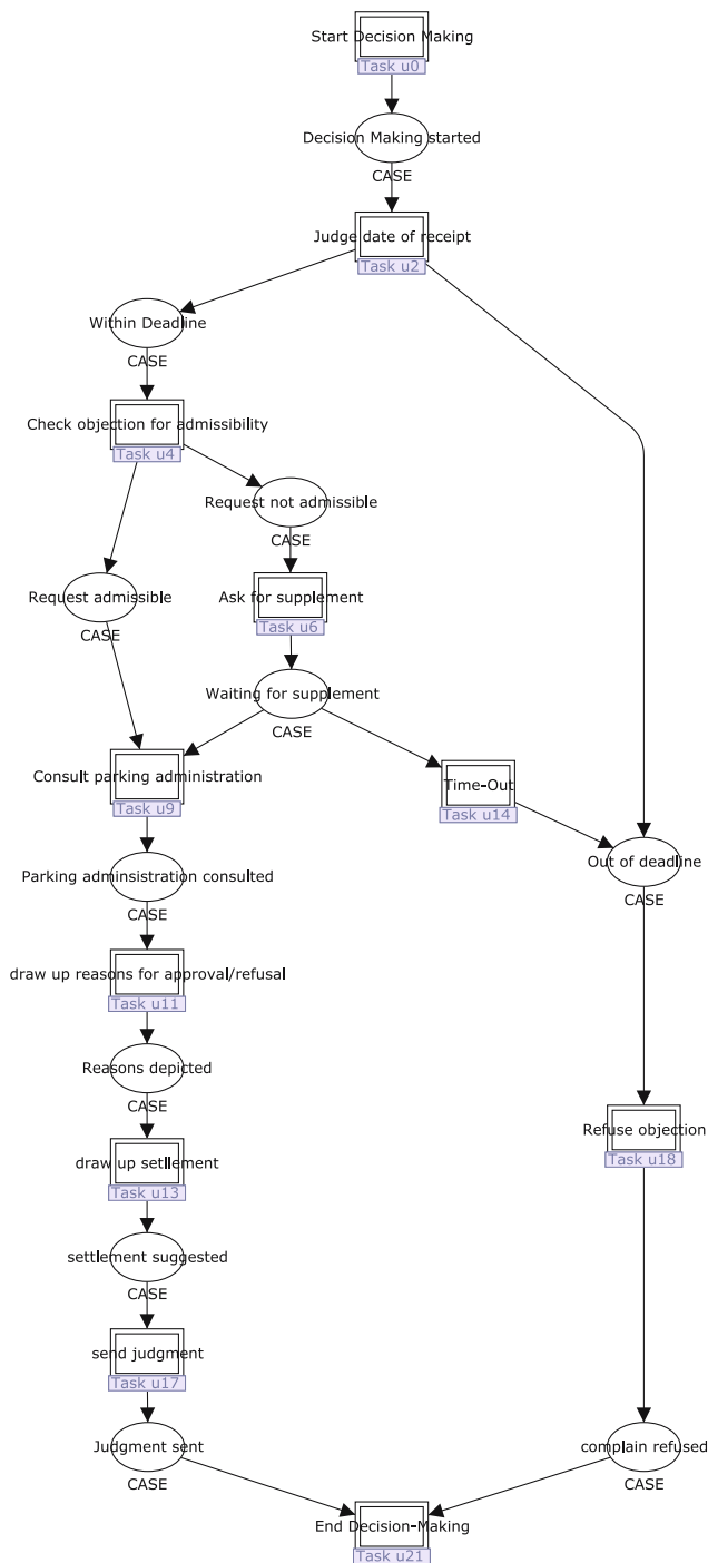
Fig. 2 The overall process model of the CPN (generated from the Protos process model depicted in Fig. 1)
