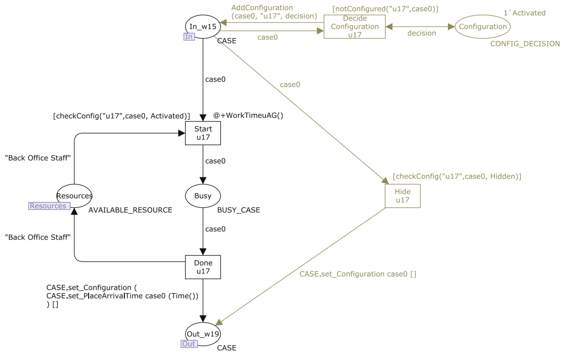
Fig. 8 A sub page of a configurable task
