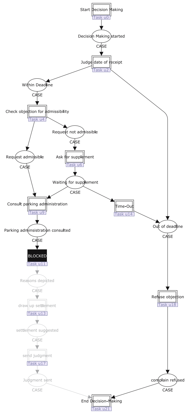
Fig. 11 Task draw up reasons for approval/refusal blocked (black)
