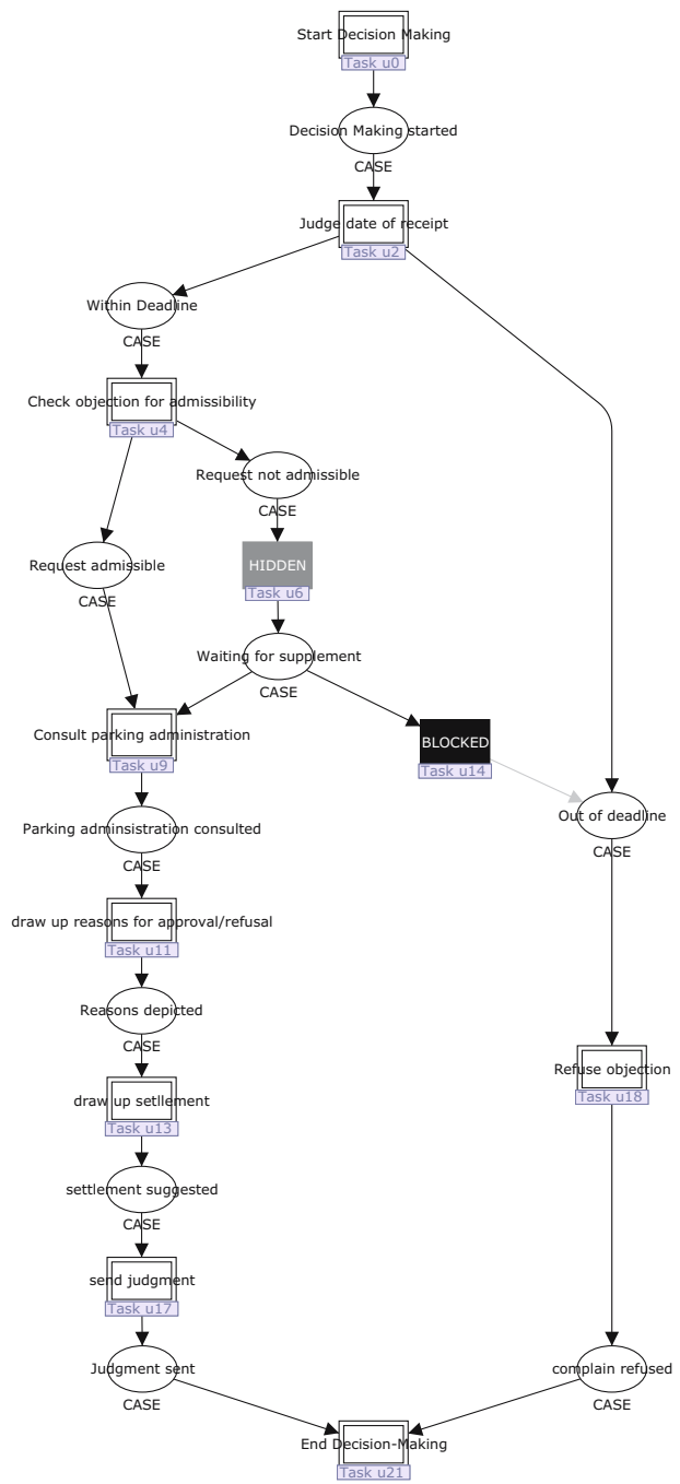
Fig. 15 To avoid asking for supplements, not only the Task Ask for supplement is hidden (grey), but also task Time-Out must be blocked (black)
