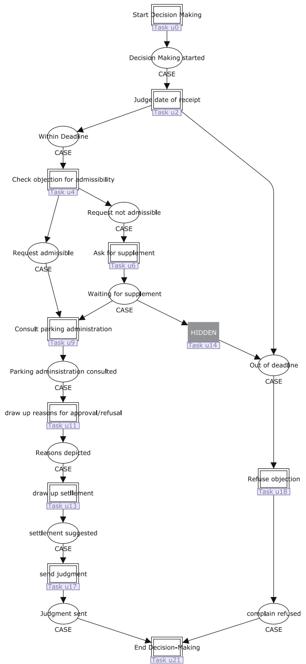
Fig. 13 Task Time-Out hidden (grey)
