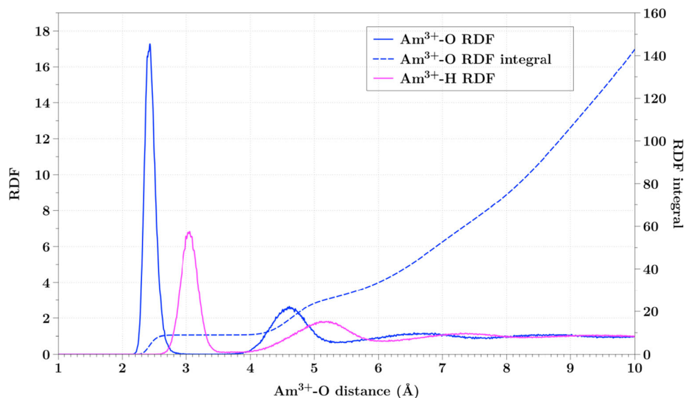
Fig. 2 Radial distribution functions (RDF) for O (and its integral) and H as a function of the \text{Am}^{3+} -O or \text{Am}^{3+} -H distance
