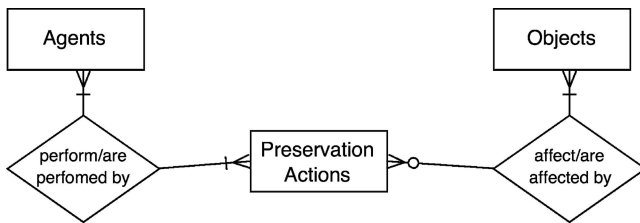
Fig. 2 Basic preservation metadata model
