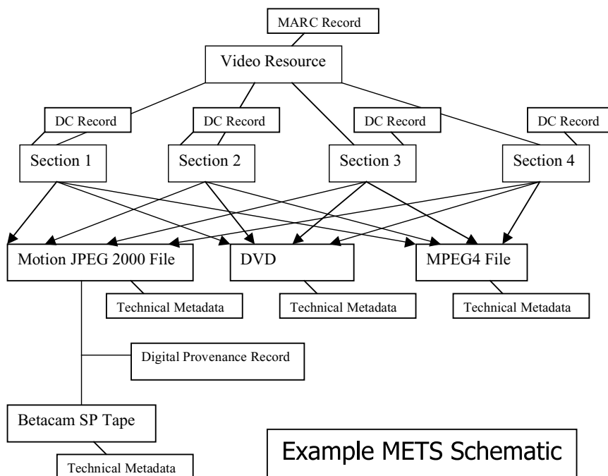
Fig. 1 Relationships tracked by METS for a typical video digital library object
