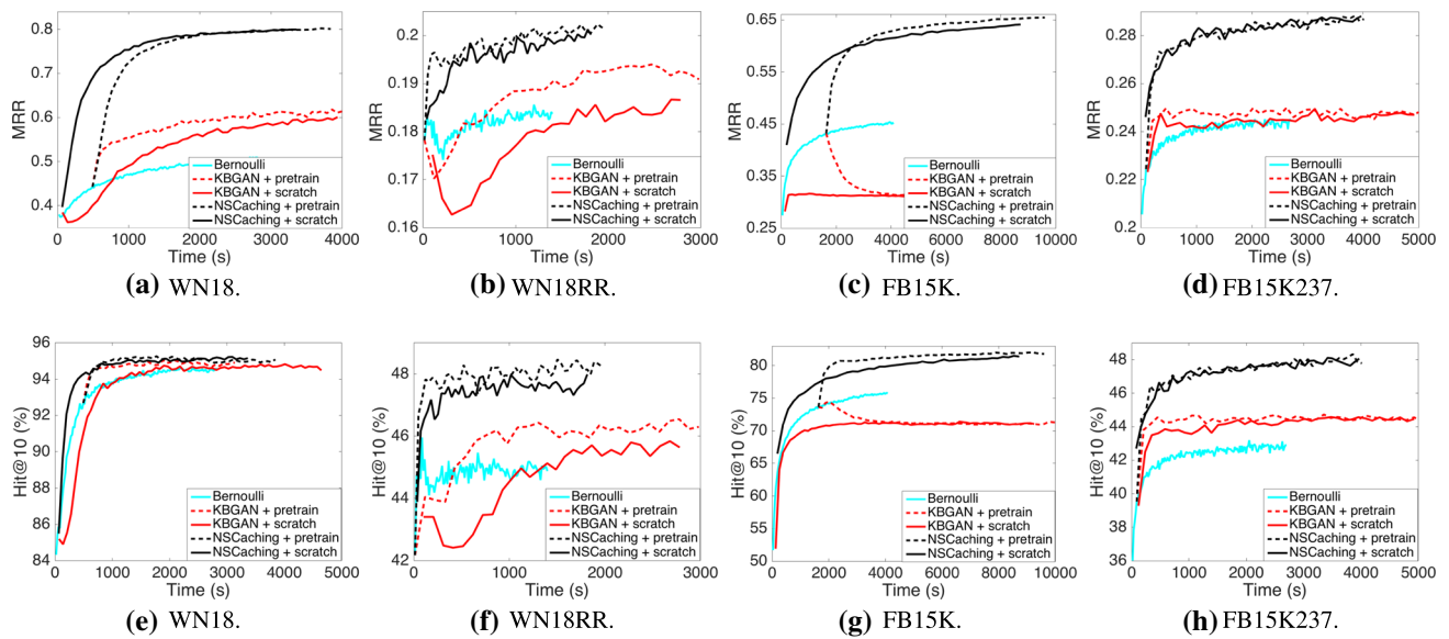
Fig. 4 Testing performance versus clock time (in seconds) based on TransD (best viewed in color) (color figure online)
