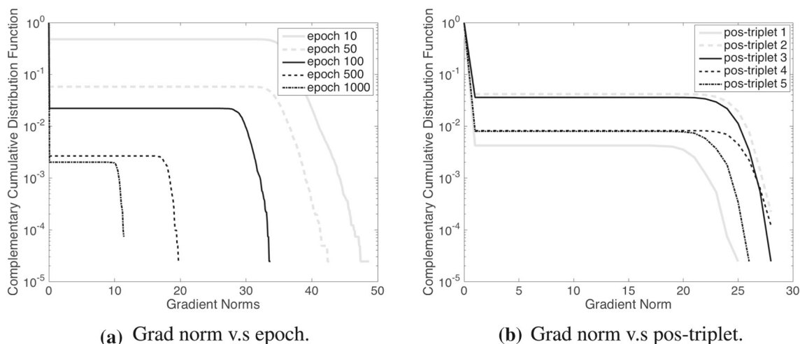
Fig. 2 Distribution of training pairs' gradients on WN18 trained by Bernoulli-TransE (see Sect. 5.3.1). For a given triplet (h_i, r_i, t_i) , we fix the head entity h and relation r and compute the \ell_2 -norm of gradient \|\mathbf{g}\|_2 in (3) for all \bar{t} \in \mathcal{E} . We measure the complementary cumulative distribution function (CCDF) F_{\|\mathbf{g}\|_2}(x) = P(\|\mathbf{g}\|_2 \geq x) to show the
