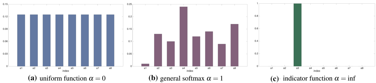
Fig. 3 Example of the different distributions of \sigma , where x -axis indicates each dimension of \mathbf{a} in (13) and y -axis is the sampling probability
