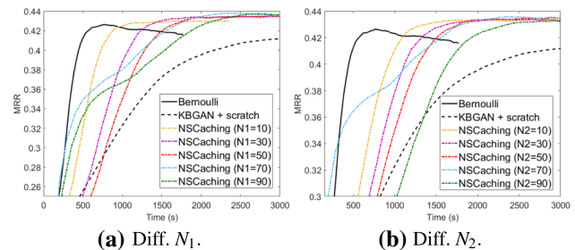
Fig. 7 Comparison of different N_1 when random subset size N_2 is fixed to 50, and different N_2 when cache size N_1 is fixed to 50. Evaluated by Simple model on WN18RR (best viewed in color) (color figure online)
