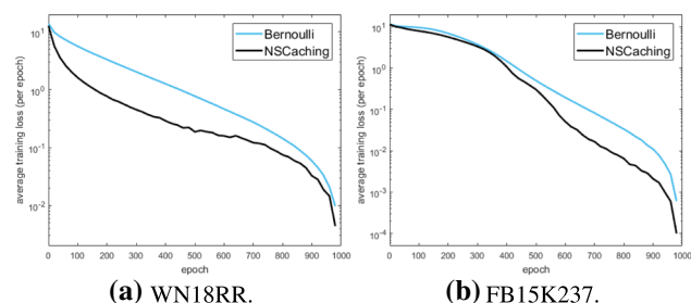
Fig. 14 Average training loss in one epoch versus number of epochs for Bernoulli and NSCaching
