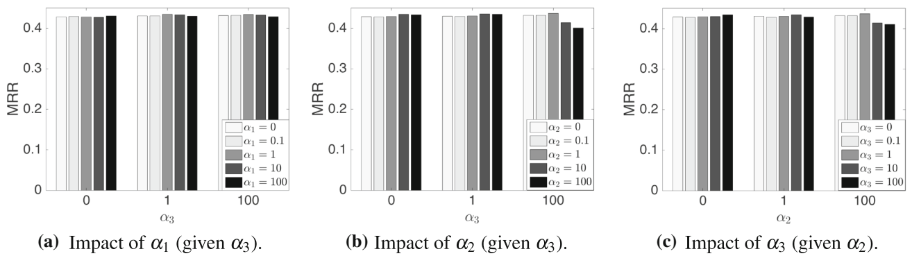
Fig. 6 Balancing on exploration and exploitation with different values of \alpha_1 , \alpha_2 and \alpha_3 with Simple on WN18RR
