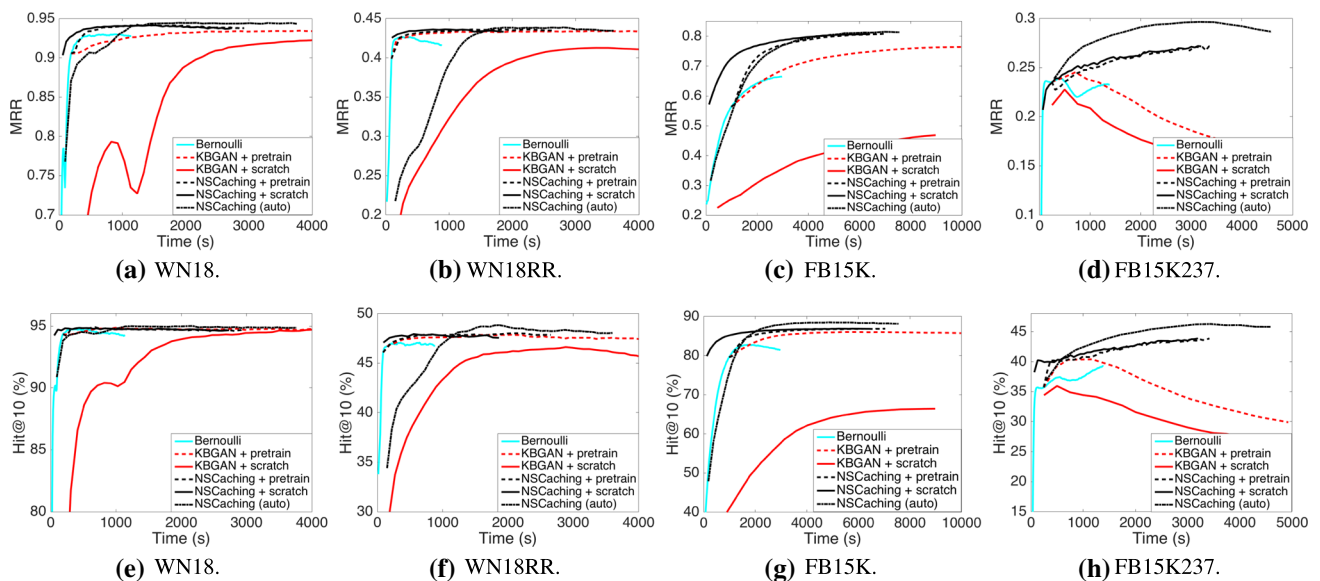
Fig. 5 Testing performance versus clock time (in seconds) based on Simple (best viewed in color) (color figure online)
