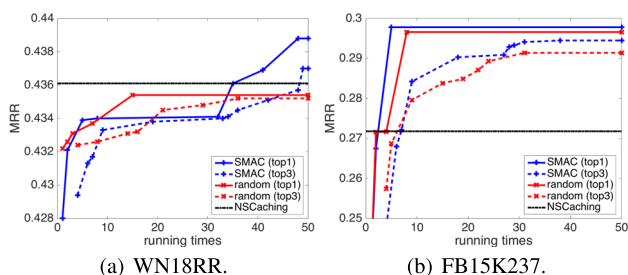
Fig. 8 Performance comparison of SMAC and random search (top1 and top3 average). x -axis is number of running times for different hyper-parameter. y -axis is the mean MRR on validation set. The MRR performance of NSCaching is given as the black-dashed line for a reference (best viewed in color) (color figure online)
