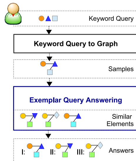
Fig. 1 Exemplar Query Answering process
