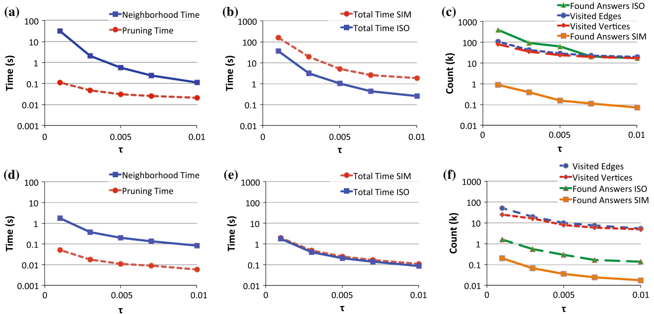
Fig. 15 Study of the average (top) and median (bottom) time and number of results (count) as a function of the threshold \tau , comparing isomorphism and simulation with the APFASTXQ/APFASTXQSIM algorithms, a average neighbor and pruning time, b average total time,
