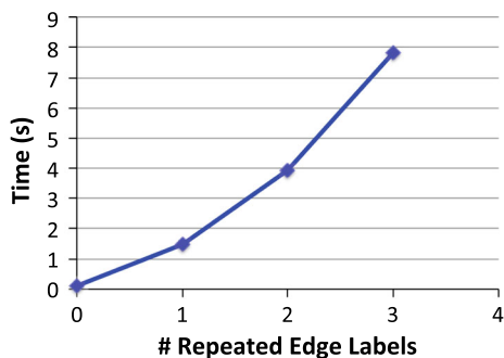
Fig. 17 Search time versus number of repeated labels
