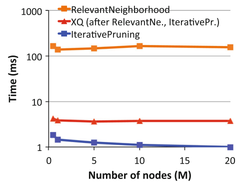
Fig. 22 Time versus number of nodes (GSize-x dataset)
