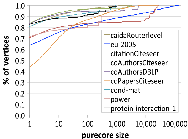
Fig. 7 Cumulative purecore size distribution for real-world graphs
