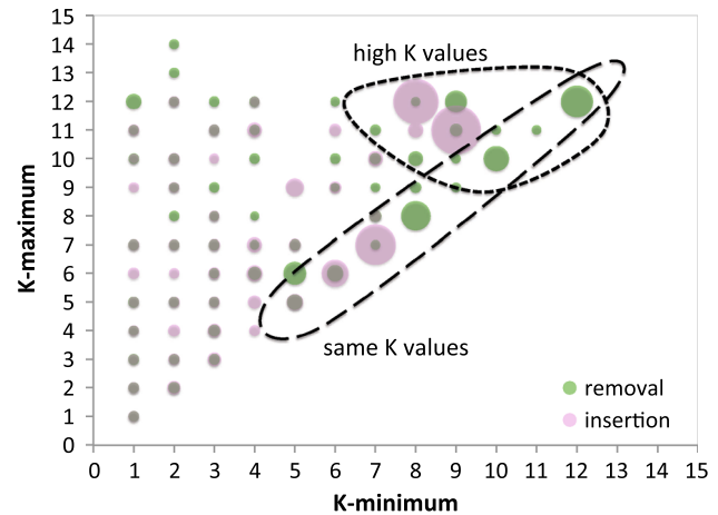
Fig. 12 Edge insertion and removal execution times of the traversal algorithm for different K values. Runtime shows low variability in general with higher runtimes when K values are high and/or equal
