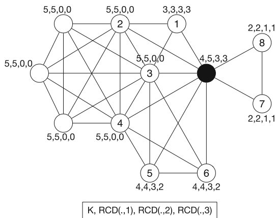
Fig. 3 Illustration of RCD values of the vertices in the sample graph from arbitrary number of hops. Accordingly, in this section, we present the generic traversal algorithm for edge insertion, which leverages the multihop residential information of vertices for potentially faster calculation of K values.
