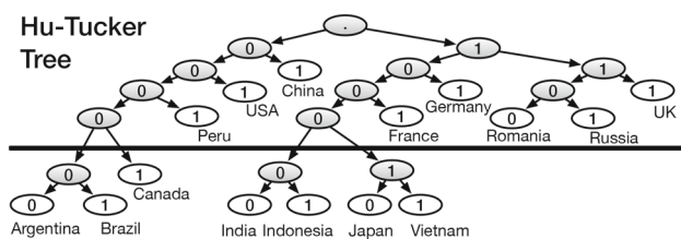
Fig. 7 Hu–Tucker tree for dimension D_NATION of Fig. 4
