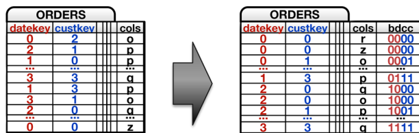
Fig. 3 Example of a BDCC table ORDERS, according to the example introduced earlier. An additional column _bdcc_ is added and ORDERS is sorted after _bdcc_
