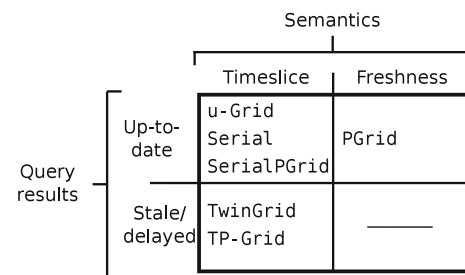
Fig. 10 Index classification
