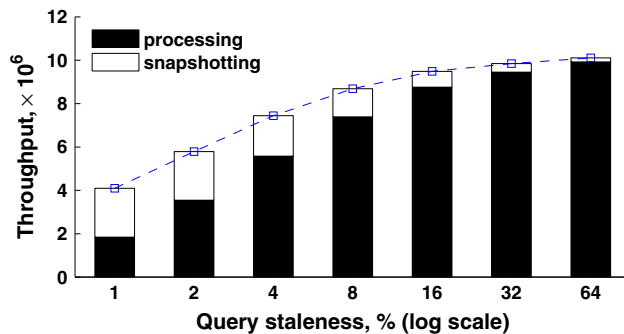
Fig. 12 Effects of varying the query staleness in TwinGrid on Ivy Bridge
