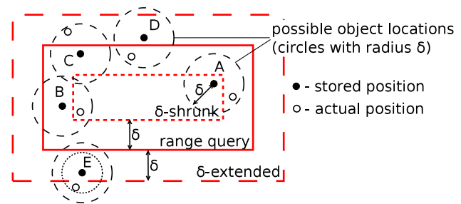
Fig. 1 Effects of extending/shrinking query range
