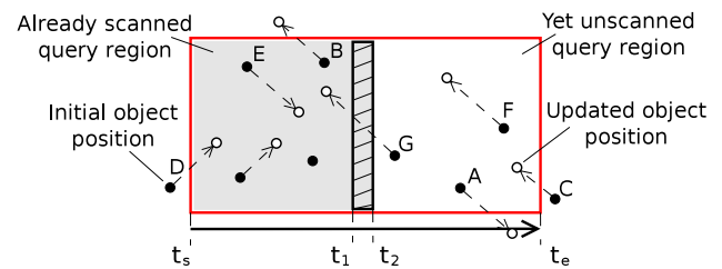
Fig. 3 Parallel updating and querying
