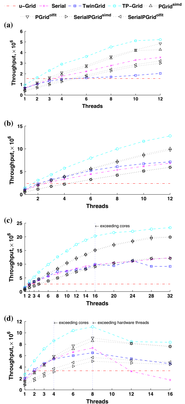
Fig. 15 Multi-threaded scalability. a 12-core Magny-Cours, b 12-core Westmere, c 16-core Sandy Bridge, d 4-core Ivy Bridge
