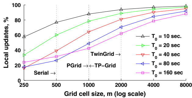
Fig. 17 Varying grid cell size and T_0
