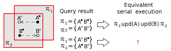
Fig. 4 Freshness semantics is not serializable
