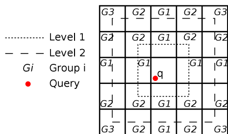
Fig. 8 Grid cell partitioning
