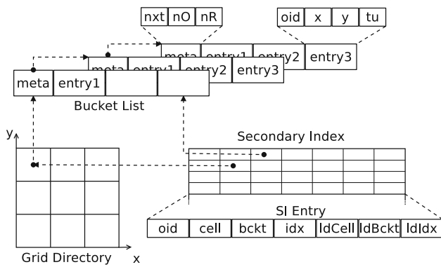
Fig. 7 Parallel grid structure
