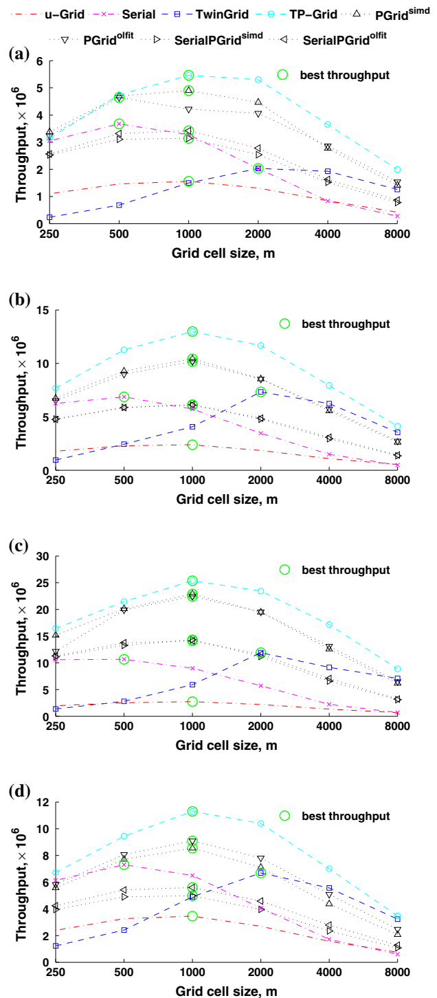
Fig. 14 Optimal grid cell size. a 12-core Magny-Cours, b 12-core Westmere, c 16-core Sandy Bridge, d 4-core Ivy Bridge
