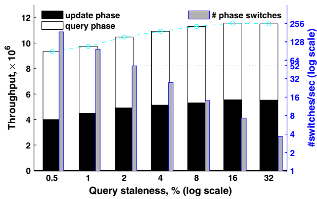
Fig. 13 Effects of varying the query staleness in TP-Grid on Ivy Bridge
