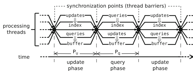
Fig. 9 Two-phase switching in TP-Grid
