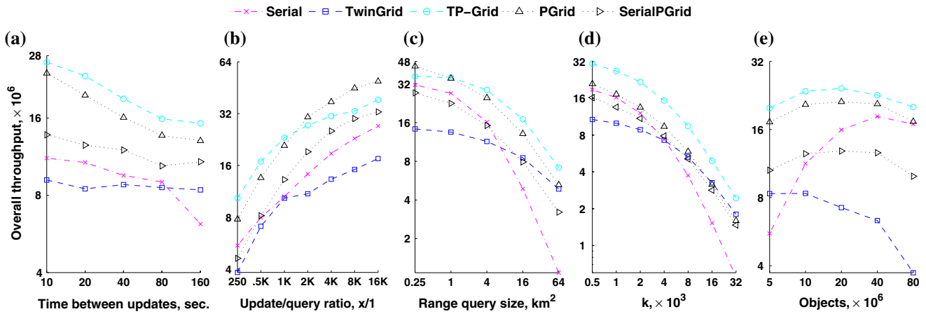
Fig. 16 Serial versus TwinGrid versus TP-Grid versus PGrid versus SerialPGrid on a 16-core Sandy Bridge machine. a Varying T_0 . b Varying update/query ratio. c Varying range query. d Varying k NN query. e Varying #objects
