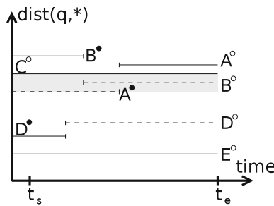
Fig. 5 3NN query with the result \{E^\circ, D^\circ, C^\circ\} , satisfying the freshness semantics
