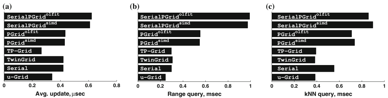
Fig. 11 Single-threaded performance. a Average CPU time per update. b Average CPU time per range query. c Average CPU time per k NN query
