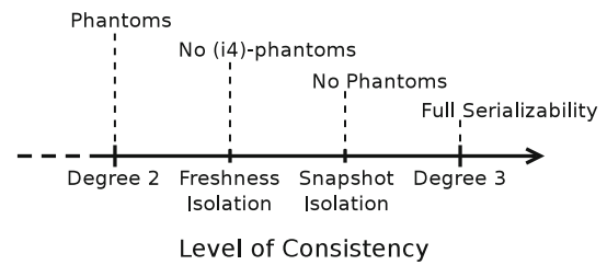
Fig. 6 Semantic relationships
