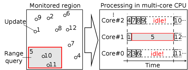
Fig. 2 Serializable processing: a long-running range query blocks rapid updates. Numbers indicate arrival order
