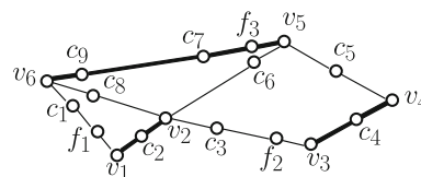
Fig. 2 Example of G
