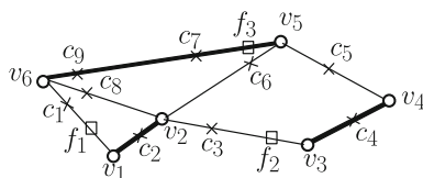
Fig. 1 Example of G^\circ
