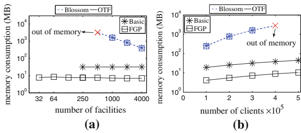
Fig. 34 Memory consumption of AddC(c) (MinMaxLQ on SF ). a Effect of |F| , b effect of |C|
