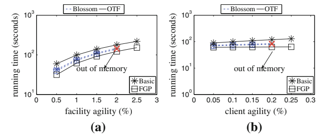
Fig. 40 COLQ Running time: effect of agility (CLQ on SF). a Effect of f_F , b effect of f_C
