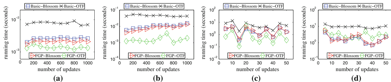
Fig. 31 Update running time: growth of updates (CLQ on SF), a AddC(c) , b DelC(c) , c AddF(f) , d DelF(f)
