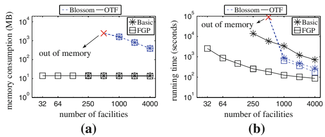
Fig. 25 Effect of |F| (MinMaxLQ on SF ). a Memory consumption, b running time
