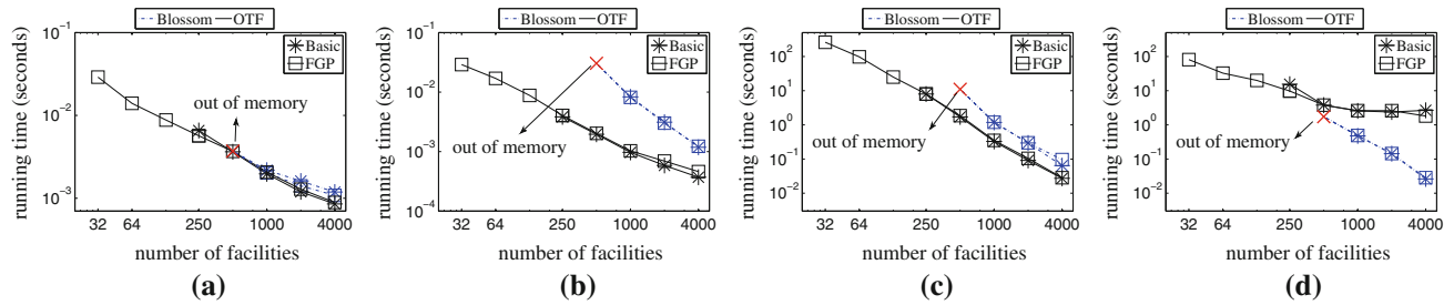
Fig. 35 Update running time: effect of |F| (MinSumLQ on SF ). a AddC(c) , b DelC(c) , c AddF(f) , d DelF(f)
