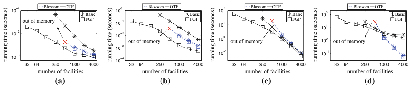
Fig. 28 Update running time: effect of |F| (CLQ on SF). a AddC(c) , b DelC(c) , c AddF(f) , d DelF(f)
