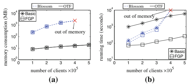
Fig. 26 Effect of |C| (MinMaxLQ on SF ). a Memory consumption, b running time
