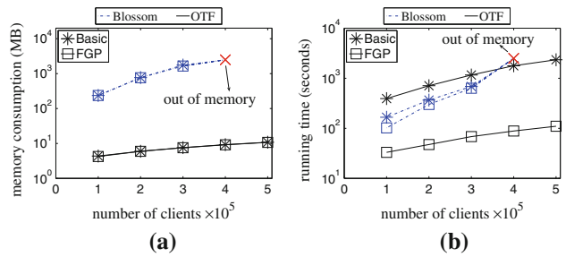
Fig. 24 Effect of |C| (MinSumLQ on SF ). a Memory consumption, b running time
