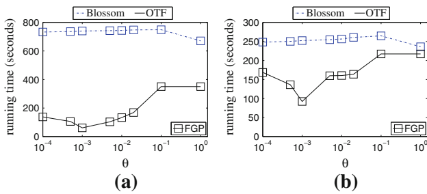
Fig. 16 Running time versus \theta (CLQ). a SF , b CA
