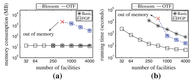
Fig. 18 Effect of |F| (CLQ on SF ). a Memory consumption, b running time
