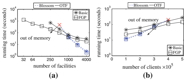
Fig. 39 COLQ Running time: effect of |F| and |C| (CLQ on SF). a Effect of |F| , b effect of |C|
