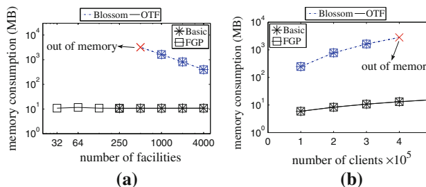
Fig. 33 Memory consumption of AddC(c) (MinSumLQ on SF), a Effect of |F| , b effect of |C|
