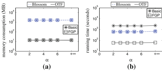
Fig. 17 Effect of \alpha (CLQ on SF ). a Memory consumption, b running time
