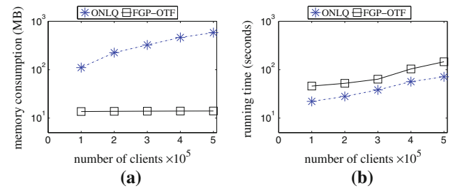
Fig. 22 Comparison with ONLQ in [10] (on SF ). a Memory consumption, b running time
