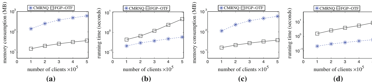
Fig. 32 Comparison with CMRNQ in [11] (on SF), a AddF(f) , b DelF(f) , c AddC(c) , d DelC(c)
