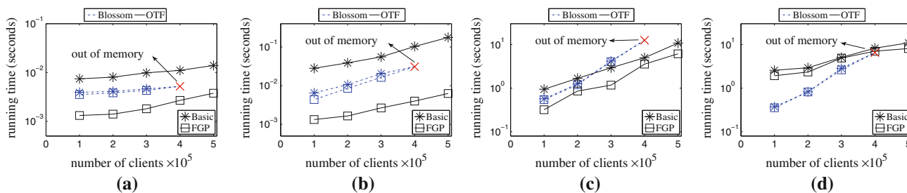
Fig. 30 Update running time: effect of |C| (CLQ on UN), a AddC(c) , b DelC(c) , c AddF(f) , d DelF(f)
