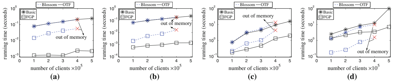
Fig. 38 Update running time: effect of |C| (MinMaxLQ on SF). a AddC(c) , b DelC(c) , c AddF(f) , d DelF(f)
