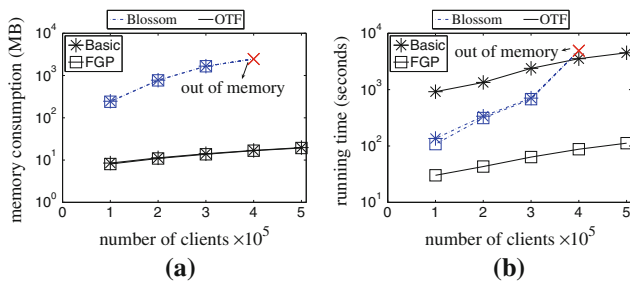
Fig. 19 Effect of |C| (CLQ on SF ). a Memory consumption, b running time
