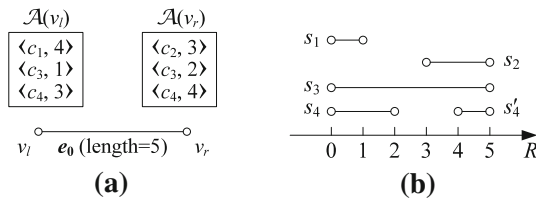
Fig. 4 Demonstration of CompLoc . a Edge e_0 , b Plane R
