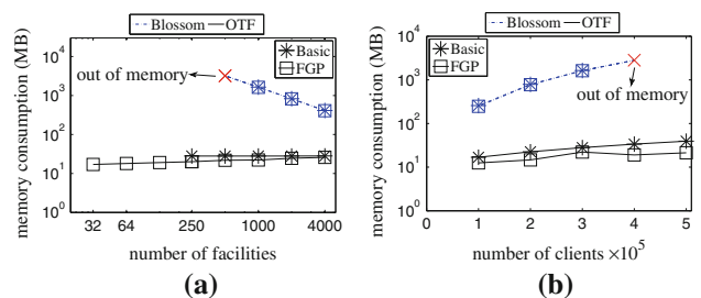
Fig. 27 Memory consumption of AddC ( c ) (CLQ on SF ). a Effect of |F| , b effect of |C|
