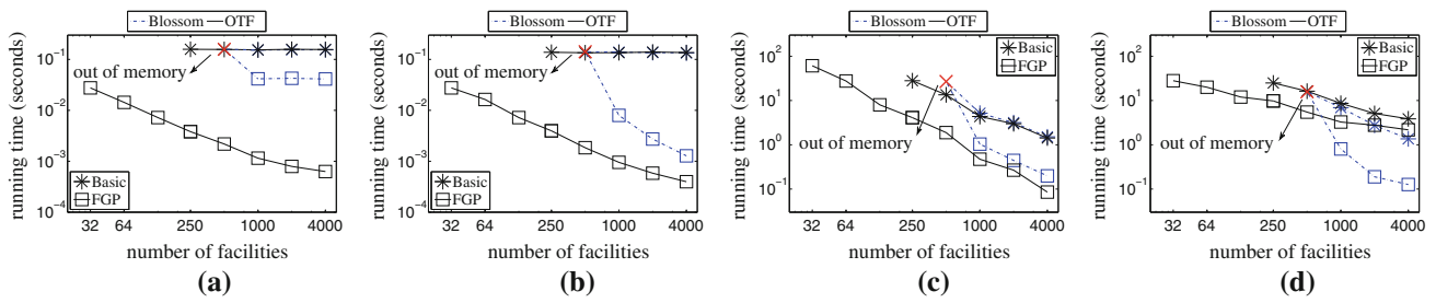
Fig. 37 Update running time: effect of |F| (MinMaxLQ on SF). a AddC(c) , b DelC(c) , c AddF(f) , d DelF(f)
