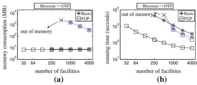
Fig. 23 Effect of |F| (MinSumLQ on SF ). a Memory consumption, b running time
