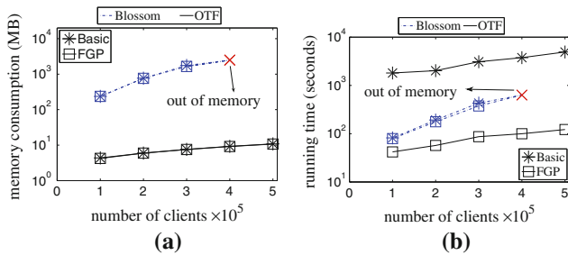
Fig. 20 Effect of |C| (CLQ on UN ). a Memory consumption, b running time
