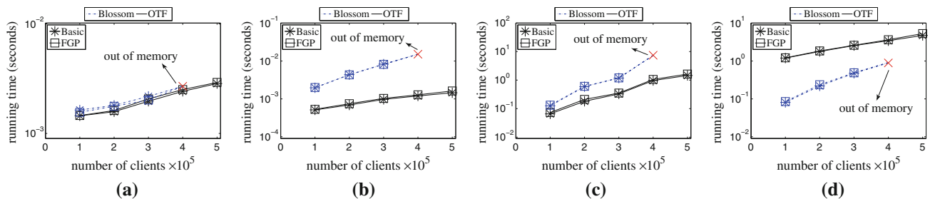
Fig. 36 Update running time: effect of |C| (MinSumLQ on SF ). a AddC(c) , b DelC(c) , c AddF(f) , d DelF(f)
