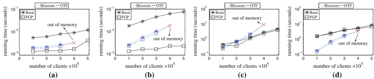
Fig. 29 Update running time: effect of |C| (CLQ on SF), a AddC(c) , b DelC(c) , c AddF(f) , d DelF(f)
