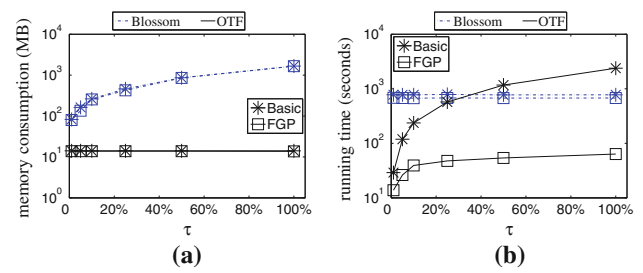
Fig. 21 Effect of \tau (CLQ on SF ). a Memory consumption, b running time
