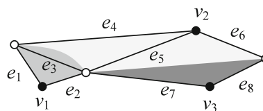
Fig. 8 Example of GPart
