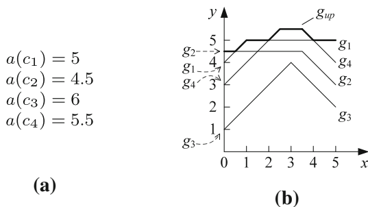
Fig. 5 Representing attractor distances as functions of the location of the new facility. a Attractor distances without the new facility, b Piecewise linear functions
