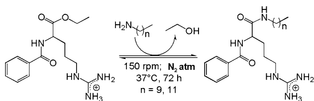
Fig. 1 Papain-catalysed syntheses of N^\alpha -benzoyl-arginine decylamide (Bz-Arg-NHC 10 ) and N^\alpha -benzoyl-arginine dodecylamide (Bz-Arg-NHC 12 )
