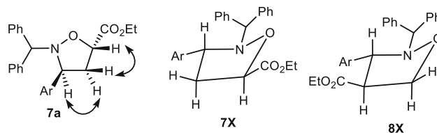
Fig. 1 Selected ROESY spectrum for ester 7a and preferred conformations of esters 7a–7c and 8a–8c
