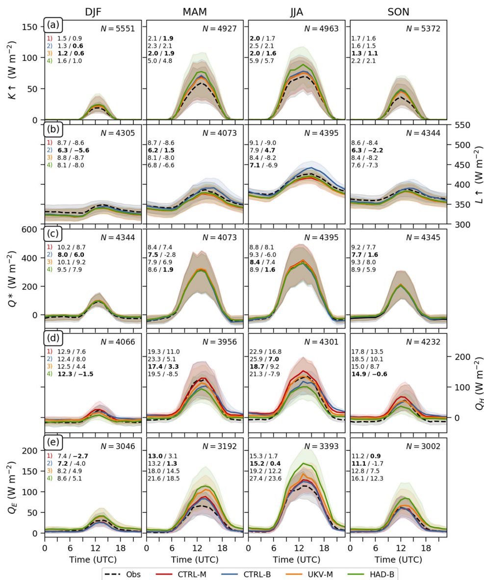
Fig. 6 As Fig. 5, but for Swindon with the seasonal 24-h MAE / MBE ( \text{W m}^{-2} ) for (1) CTRL-M, (2) CTRL-B, (3) UKV-M, (4) HAD-B
