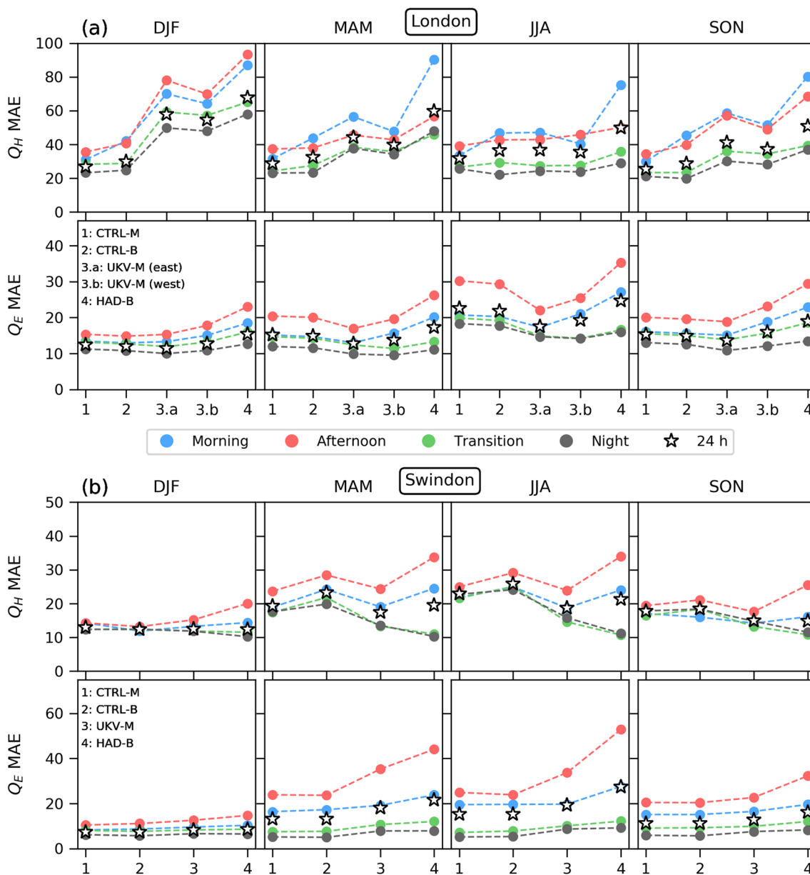
Fig. 7 MAE ( W m^{-2} ) of Q_H and Q_E for (a) London/KCL and (b) Swindon per season and by time-of-day (Section 5.2) for each model configuration. Dashed lines are used for ease of visualising relations between model configurations. 24-h values (stars) are given in Figs. 5 and 6
