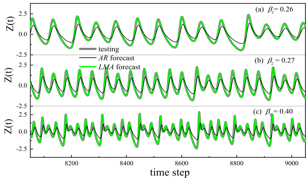
Fig. 8 Comparison between predicted time series (black lines from AR(4) and green lines from LMA) and testing chaotic time series (gray lines) with different nonlinearity: (a) 0.26, (b) 0.27, and (c) 0.40
