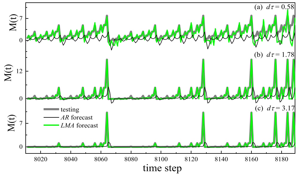
Fig. 6 Comparison between predicted time series (black lines from AR(4) and green lines from LMA) and testing multifractal time series (gray lines) with different multifractal strengths: (a) 0.58, (b) 1.78, and (c) 3.17
