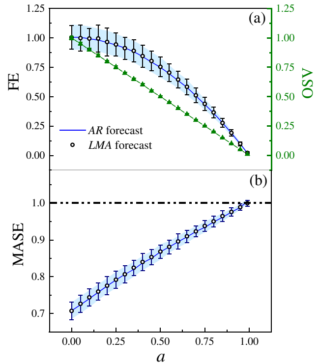
Fig. 3 Evaluation of predicted time series with short-term memory: (a) FE and (b) MASE. The solid blue lines present AR predictions (blue shadows behind are intervals of 2.5 standard deviation) and hollow black dots represent LMA predictions (error bars are intervals of 2.5 standard deviation). In particular, the solid green up-triangles represent the variation of one-step variability in chaotic time series
