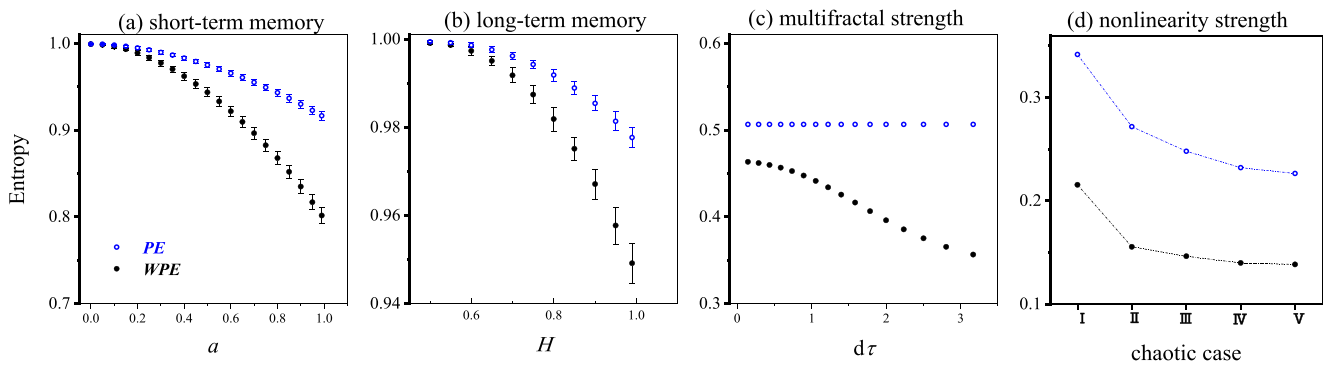
Fig. 1 Scatter plots for the monotonous relation between PE/WPE (hollow blue/solid black dots) and the strengths of ordinal structures with (a) short-term memory, (b) long-term memory, (c) multifractal patterns, and
