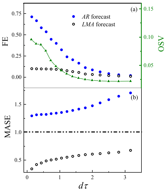
Fig. 7 Evaluation of predicted multifractal time series under different multifractal strengths: (a) FE and (b) MASE. The solid blue dots represent AR predictions and hollow black dots represent LMA predictions. In particular, the solid green up-triangles represent the variation of one-step variability in chaotic time series
