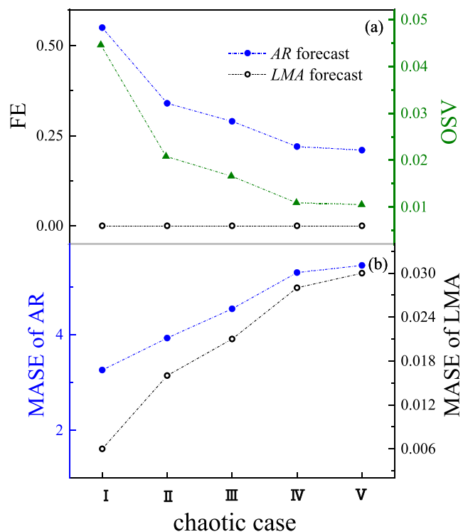
Fig. 9 Evaluation of predicted chaotic time series under different nonlinearity: (a) FE and (b) MASE. The solid blue dots represent AR predictions and hollow black dots represent LMA predictions. In particular, the solid green up-triangles represent the variation of one-step variability in chaotic time series
