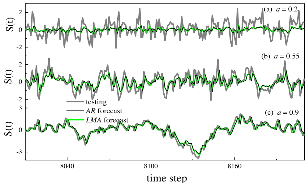
Fig. 2 Comparison between predicted time series (black lines from AR(4) and green lines from LMA) and testing time series with different long-term memory (gray lines): (a) 0.2, (b) 0.55, and (c) 0.9
