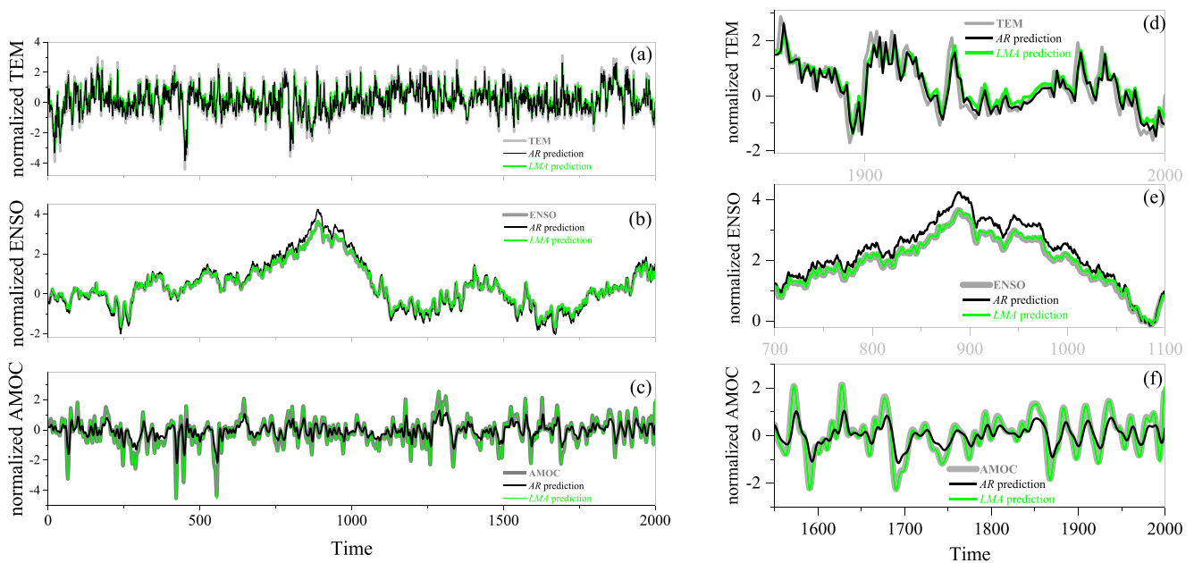
Fig. 11 Comparison between predicted time series (black lines from AR(4) and green lines from LMA) and testing real-world time series: (a) TEM, (b) ENSO, and (c) AMOC. (d)–(f) Locally enlarged version for (a)–(c), respectively
