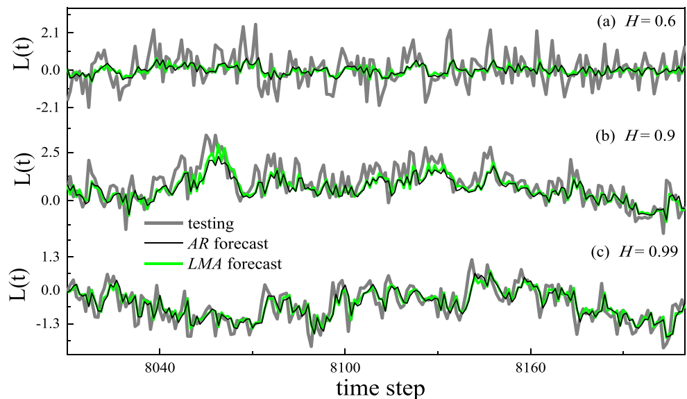
Fig. 4 Comparison between predicted time series (black lines from AR(4) and green lines from LMA) and testing time series with different long-term memory (gray lines): (a) 0.6, (b) 0.9, and (c) 0.99
