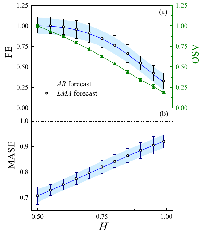
Fig. 5 Evaluation of predicted time series with different long-term memory: (a) FE and (b) MASE. The solid blue lines present AR predictions (blue shadows behind are intervals of 2.5 standard deviation) and hollow black dots represent LMA predictions (error bars are intervals of 2.5 standard deviation). In particular, the solid green up-triangles represent the variation of one-step variability in chaotic time series
