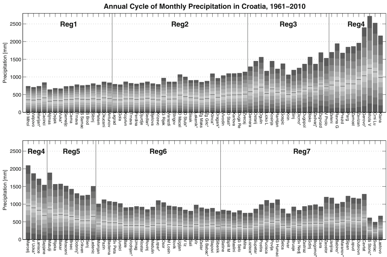
Fig. 2 Annual cycle of monthly precipitation (depicted in shades of grey) in Croatia, 1961–2010. Shortened station names correspond to names from Table A1 in Zahradniček et al. (2014). Stations with possible inhomogeneities which are not supported by metadata are denoted with an asterisk
