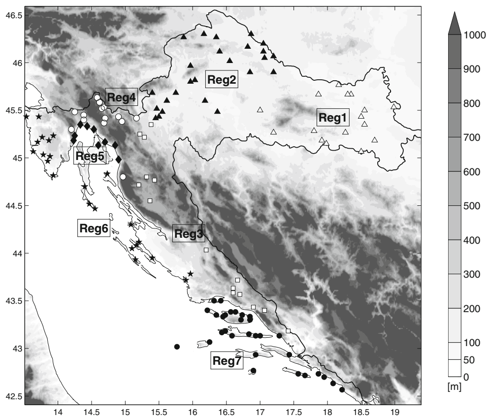
Fig. 1 Locations of the meteorological stations and regions mentioned in the text and Table 1. The orography is depicted in shades of grey
