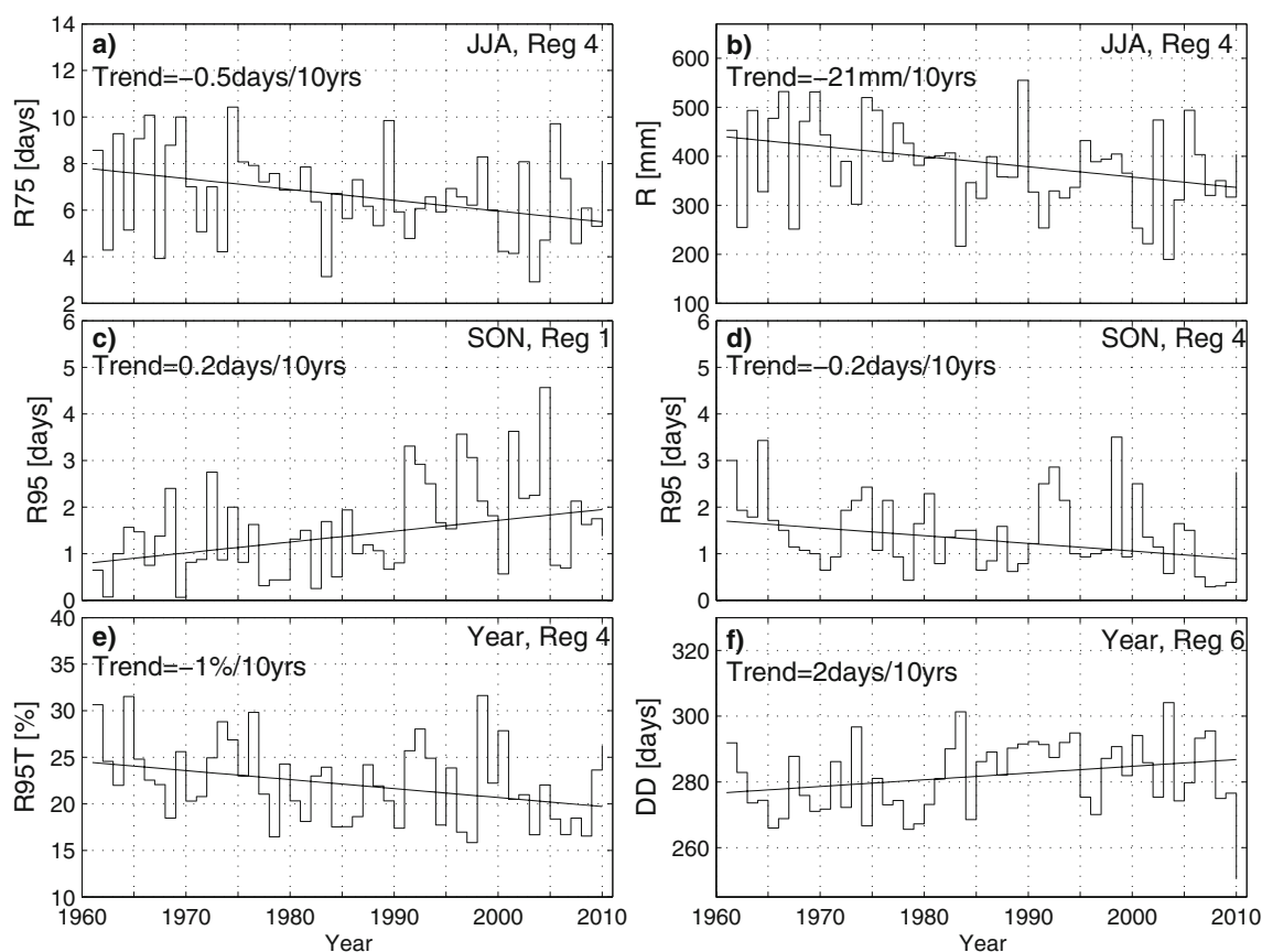
Fig. 3 Examples of regional time series with statistically significant trends. a R75 for JJA and region Reg4, b R for JJA and region Reg4, c R95 for SON and region Reg1, d R95 for SON and region Reg4, e R95T for the whole year and region Reg4 and f DD for the whole year and region Reg6
