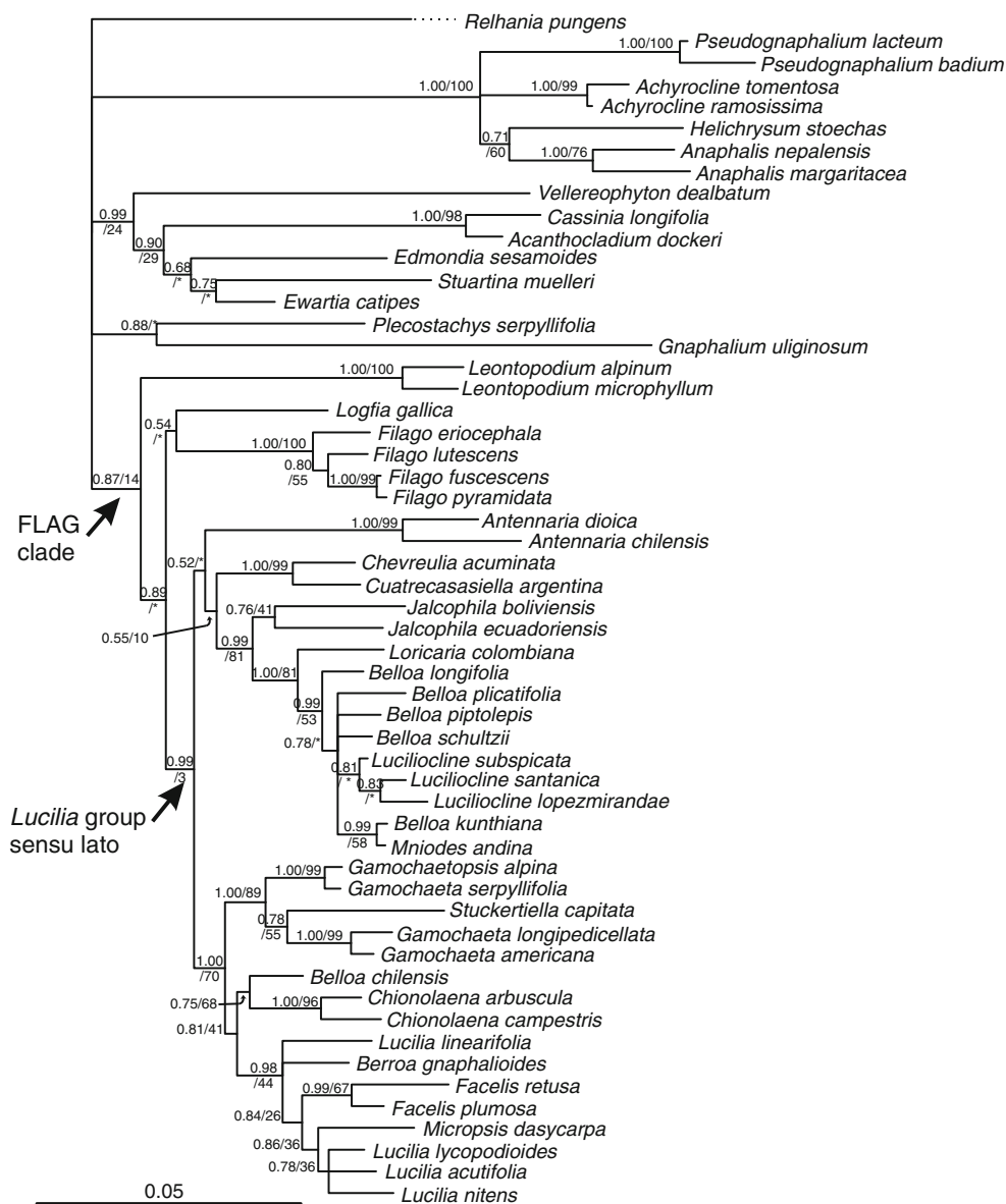
Fig. 1 Consensus phylogram obtained from the Bayesian analysis of ITS + ETS sequences (nuclear markers). Bayesian posterior probabilities (PP) and Jackknife values from the parsimony analyses are shown associated with the branches. An asterisk indicates a branch missing from the parsimony analysis. Dotted branches were shortened to have a clearer topology
