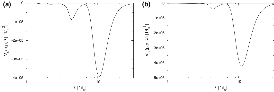
Fig. 4 a Diagonal element V(p, p, \lambda) in dependence of \lambda for p \approx 0.84 l_0^{-1} . b V'(p, p, \lambda) from Eq. (22) in dependence of \lambda for p \approx 0.84 l_0^{-1} . The parameters of the potential are \nu = 9 and \Lambda = 20 l_0^{-1} . The evolution was carried out with the standard T generator
