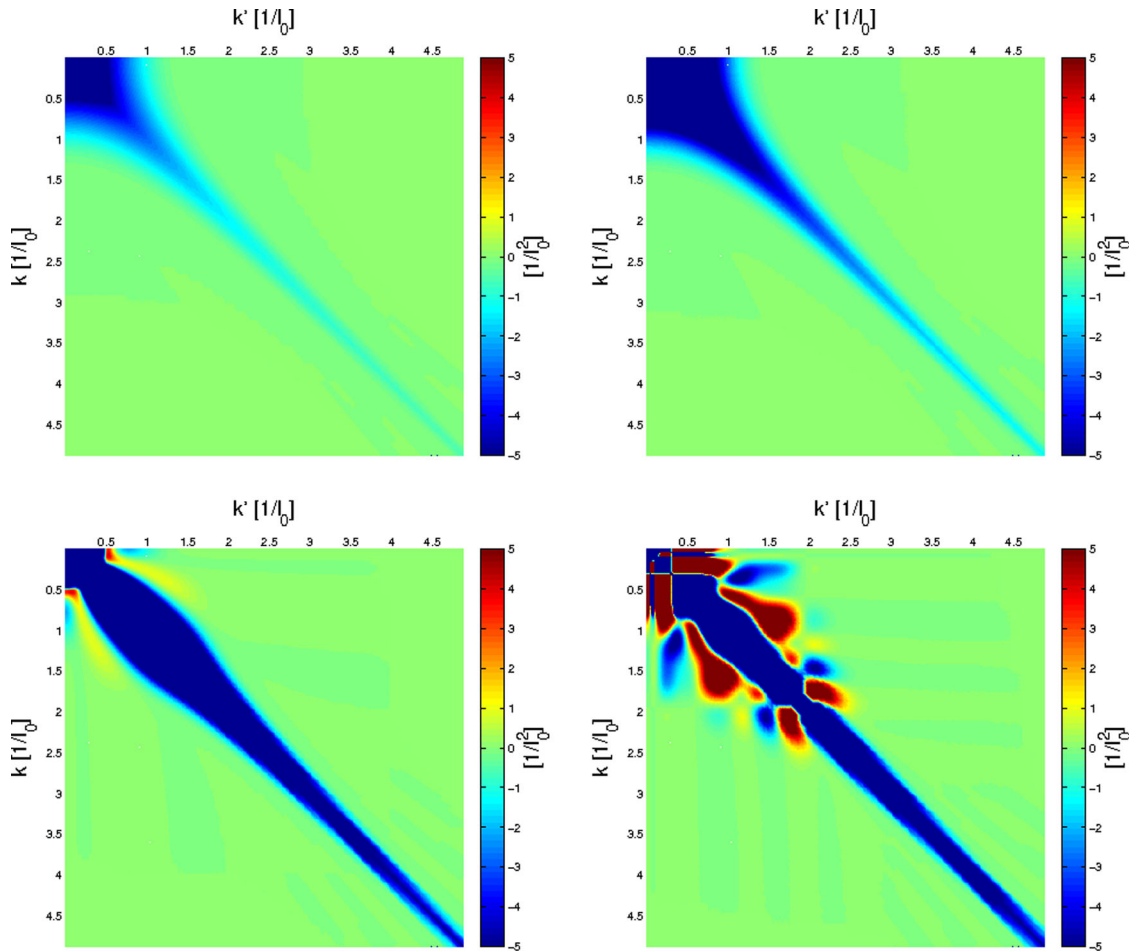
Fig. 2 S-wave 1/R^2 potential evolved with the T generator to \lambda = 1 l_0^{-1} with initial \Lambda = 20 l_0^{-1} . The potential strengths are c = -0.125 , c = -0.25 , c = -0.25 - 1^2 and c = -0.25 - 2^2 in the order from top left to bottom right
