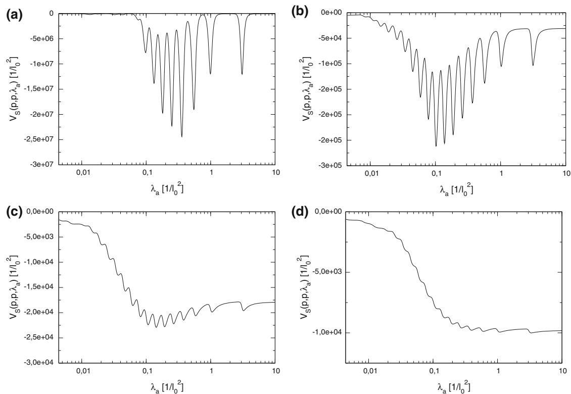
Fig. 6 Diagonal elements V(p, p, \lambda_a) evolved with the inverse generator for four different momenta p with constants \nu = 11 , \Lambda = 30 l_0^{-1} and \sigma = 0.05 l_0^{-1} : a p \approx 0.96\sigma , b p \approx 1.55\sigma , c p \approx 2.68\sigma , d p \approx 4.88\sigma
