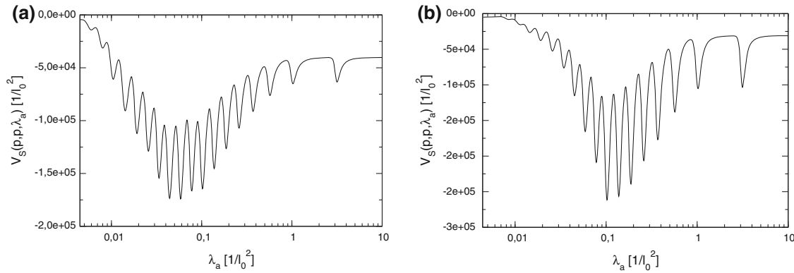
Fig. 5 Evolution of the diagonal elements V(p, p, \lambda_a) with \nu = 11 , \Lambda = 30 l_0^{-1} and \sigma = 0.05 l_0^{-1} . a Applied exponential generator with p \approx 1.19\sigma . b Applied inverse generator evolved with p \approx 1.55\sigma
