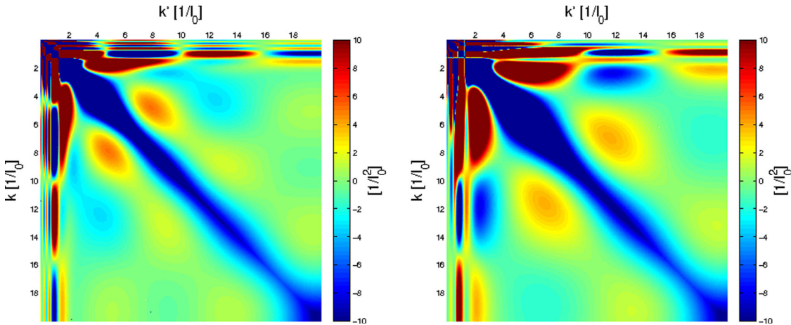
Fig. 3 Evolved 1/R^2 potential with parameters \nu = 9 , \Lambda = 20 l_0^{-1} and \sigma = 2 l_0^{-1} for G_e and G_i . Left panel evolution with the exponential generator G_e to \lambda_a \approx 8.35 l_0^{-1} . Right panel evolution with the inverse generator G_i to \lambda_a \approx 10.75 l_0^{-1}
