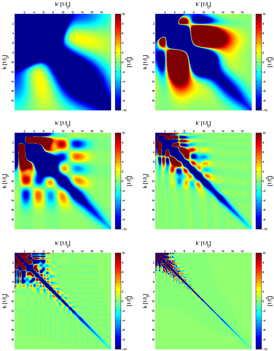
Fig. 1 Evolution of the S-wave 1/R^2 potential for the T generator with \nu = 9 and initial cutoff \Lambda = 20 l_0^{-1} . V(k, k', \lambda) is shown for \lambda \approx 21.09, 13.67, 8.86, 5.74, 3.72 and 2.41 in units of [1/l_0] from top left to bottom right
