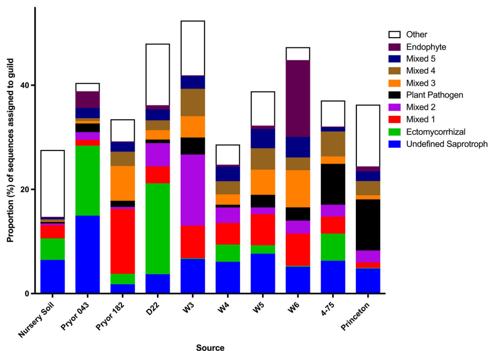
Fig. 1 Assignment of the sequence data to the most commonly encountered fungal ecological guilds using FUNGuild (Nguyen et al. 2016). OTUs with no assignment were omitted for better visualization. Guilds listed here are as follows: 1, undefined saprotroph; 2, ectomycorrhizal; 3, mixed 1: animal pathogen-endophyte-epiphyte-plant pathogen; 4, mixed 2: plant pathogen-soil saprotroph-wood saprotroph; 5, plant pathogen; 6, mixed 3: animal endosymbiont-undefined saprotroph; 7, mixed 4: animal pathogen-endophyte-epiphyte-undefined saprotroph; 8, mixed 5: animal pathogen-endophyte-plant pathogen-wood saprotroph; 9, endophyte; 10, other guilds
