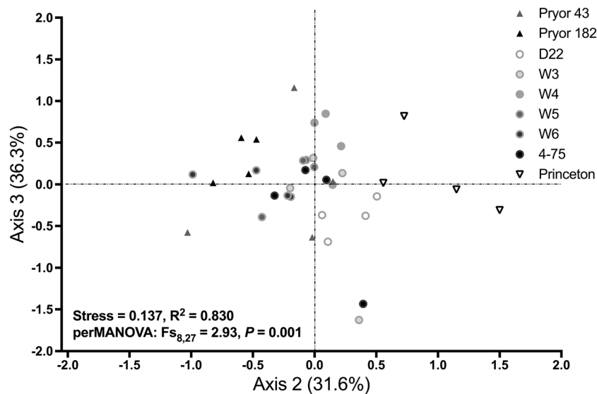
Fig. 2 Non-metric multidimensional scaling (NMS) ordination of the core fungal communities that include only those 90 OTUs that occurred at least in half of the 36 chestnut rhizobiome samples. The ordination was optimally resolved on three axes that represent 15.1%, 31.6%, and 36.3% of the variability, for a total of 83.0% with stress 0.14. The permutation-
