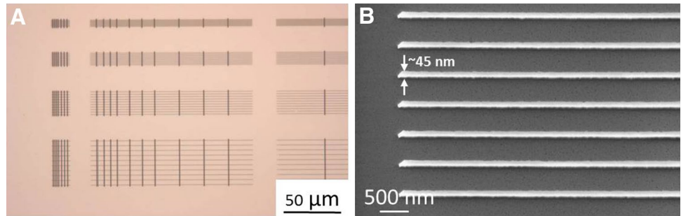
Fig. 5 a Optical microscope picture of the structures released at -8^{\circ}\text{C} and a, b SEM image of an array of lines with \sim 45 nm-width released at the same temperature
