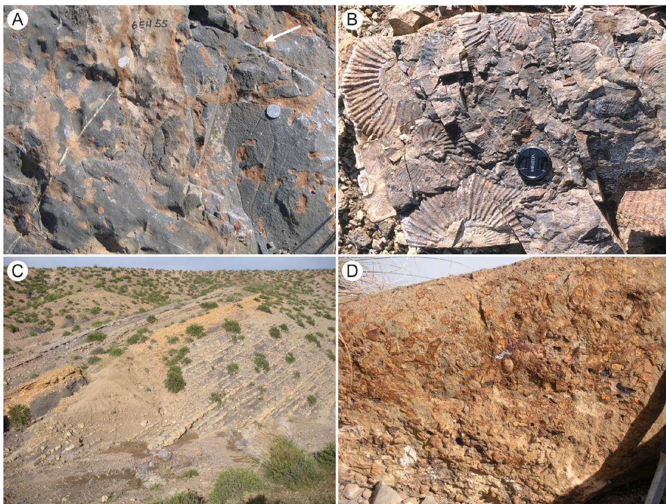
Fig. 9 Photographs of some sedimentary discontinuities observed in the Early Albian succession. a Karstic surface: Hameima Fm, Jebel Bou el Haneche section, m. 118. b Accumulation of ammonites: Fahdene Fm, Hameima section, m. 103. c Thick yellow sand bed: Fahdene Fm, Jebel Slata section, m. 446. d Matrix-supported conglomerate, with rounded calcareous clasts coated by iron oxides: Fahdene Fm, base of the Upper Albian series, Eastern flank of Jebel Slata
