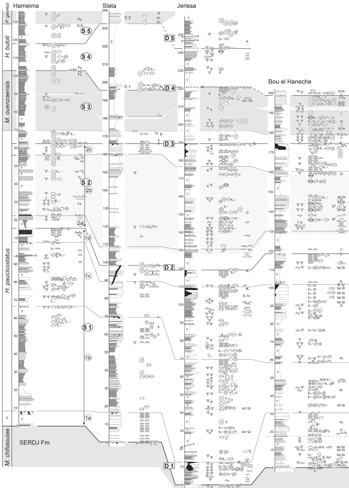
Fig. 4 Sections of the Hameima Fm and base of the Fahdene Formation in the Tajerouine area: lithology, sedimentary features and correlations. Grey area: ammonite zones (time equivalence). Dotted area: sandy interval. Location on Fig. 3. Caption on Fig. 5
