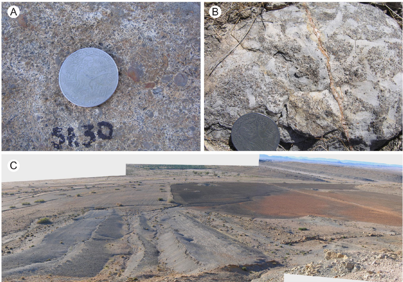
Fig. 11 Field photographs of the Fahdene Formation. a Phosphate-rich, poorly sorted calcarenite, Slata section, m. 257 (C3 on Fig. 5). b Bioturbated phosphate-rich calcarenite, Slata section, m. 314 (C4 on Fig. 5). c Marly base of S5, Hameima section, m. 190–250 (top to the right)
