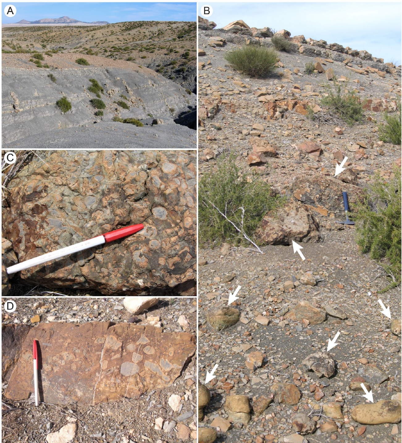
Fig. 10 Photographs illustrating the formation of phosphate-rich calcareous clasts in the Fahdene Fm. a Vertical calcareous concretions, Jebel Slata section, m. 435–450. Note the overlying reddish sandstone underlining the Late Albian transgression. b Loose and in situ septarian calcareous concretions (white arrows), El Goussa section, m.
