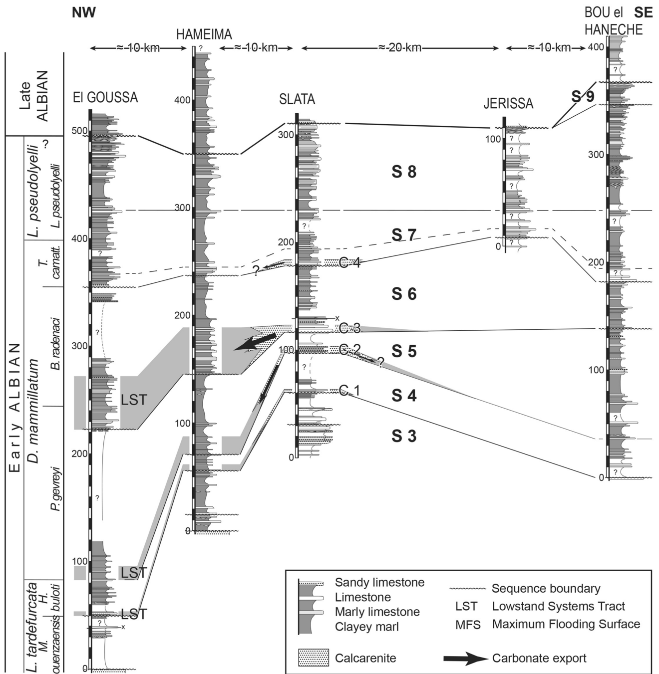
Fig. 7 Correlations of the sections studied in the Tagerouine area
