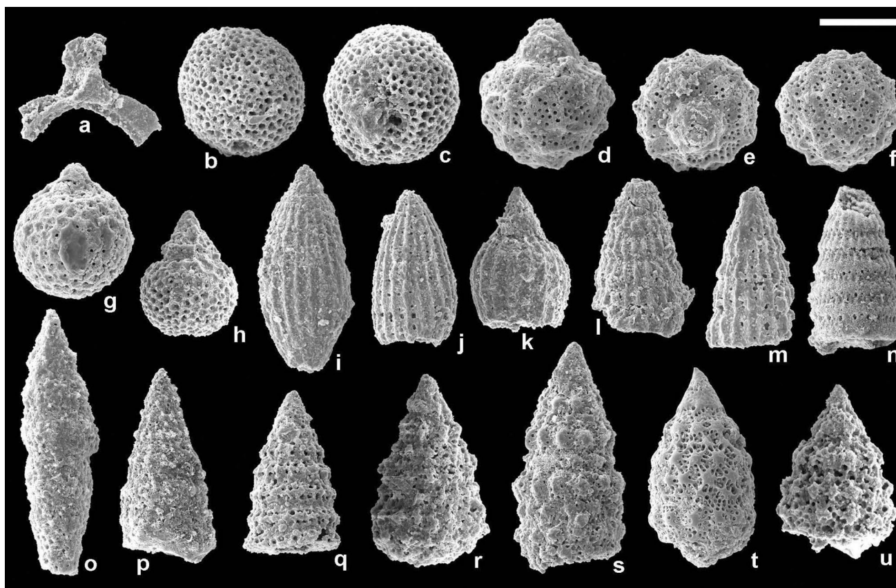
Fig. 7 Barremian radiolarians from the Studor formation of the eastern Krn Nappe. a Dicerosaturnalis trizonalis (Rüst). b, c Holocryptocanium barbui Dumitrica, apical ( b ) and antapical ( c ) view of the same specimen. d–f Arcanicapsa sp., lateral ( d ), apical ( e ) and antapical ( f ) view of the same specimen. g Hemicryptocapsa sp. h Crococapsa uterculus (Parona). i Archaeodictyomitra lacrimula (Foreman). j Archaeodictyomitra sp. k Thanarla pacifica Nakaseko
