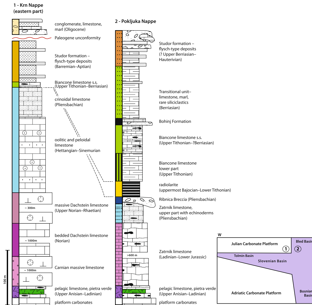
Fig. 3 Synthetic stratigraphic columns for the mapped area in the Julian Alps. Colored patterns of each stratigraphic unit correspond to the symbols in the map (Fig. 4). Inset figure: local paleogeographic sketch for the Late Triassic with location of columns 1 and 2
