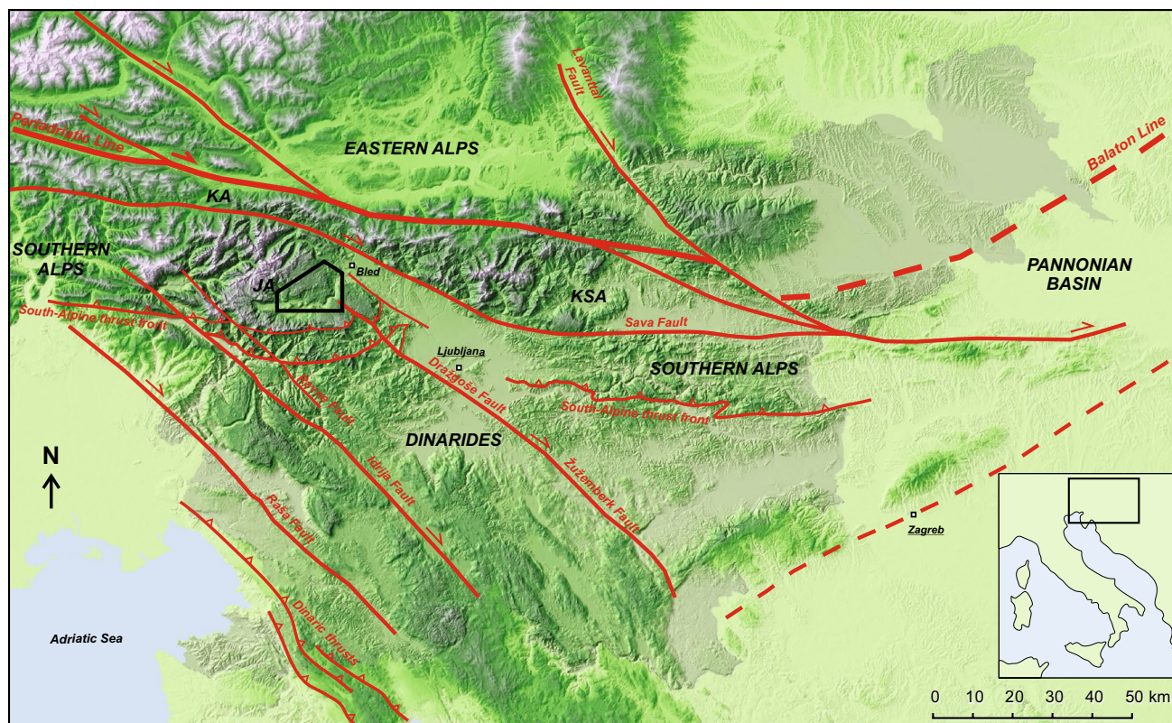
Fig. 1 Eastern Southern Alps and adjacent tectonic units (based on Placer 1999, 2009; Vrabec and Fodor 2006). The area west of Bled is enlarged in Fig. 2a, the framed polygon marks the location of the
