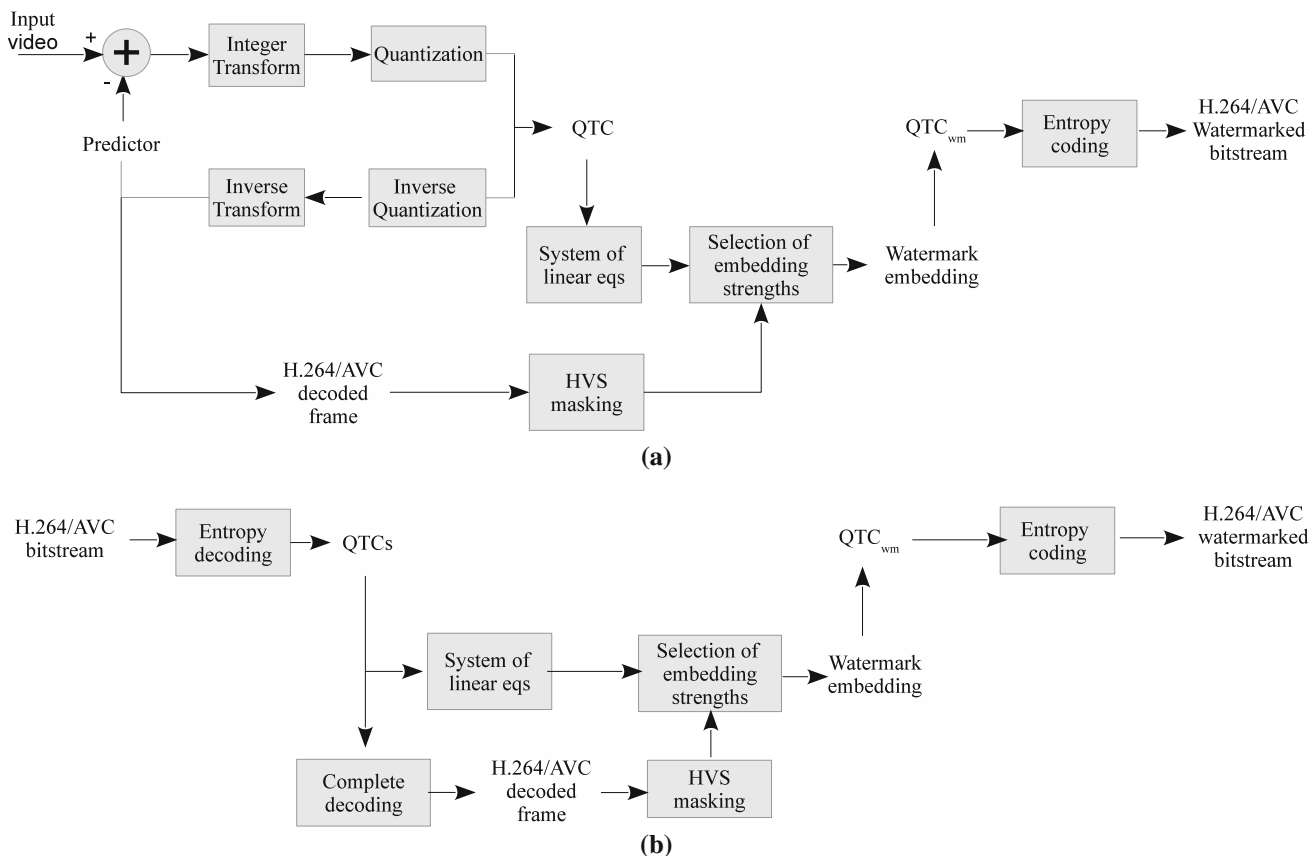
Fig. 5 Block diagram of drift-free robust watermarking system for H.264/AVC, a raw video input, and b H.264 bitstream input
