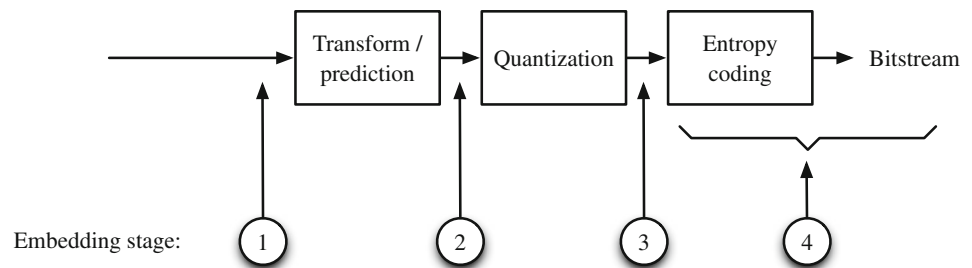
Fig. 2 Classification of watermarking schemes on the basis of working domain: (1) pre-compression, (2) transform domain, (3) quantized transform domain, and (4) open-loop
