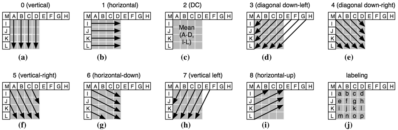
Fig. 4 Nine intra-prediction modes (a– i) and labeling of the pixels (j)
