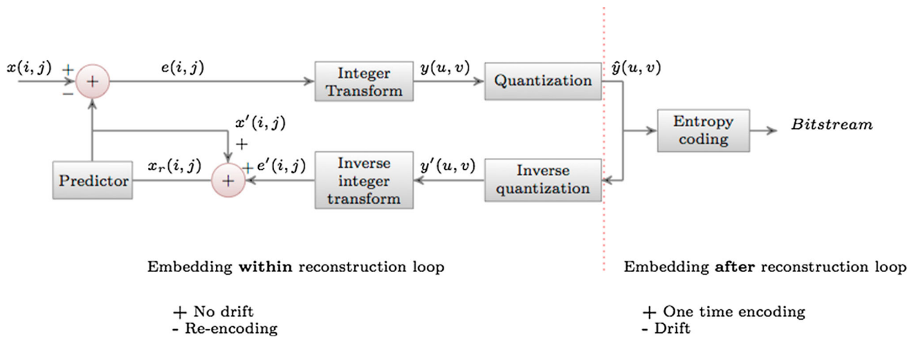
Fig. 1 Two main categories of watermarking in video codec: (1) during the encoding process or spatial domain and (2) in the bitstream domain
